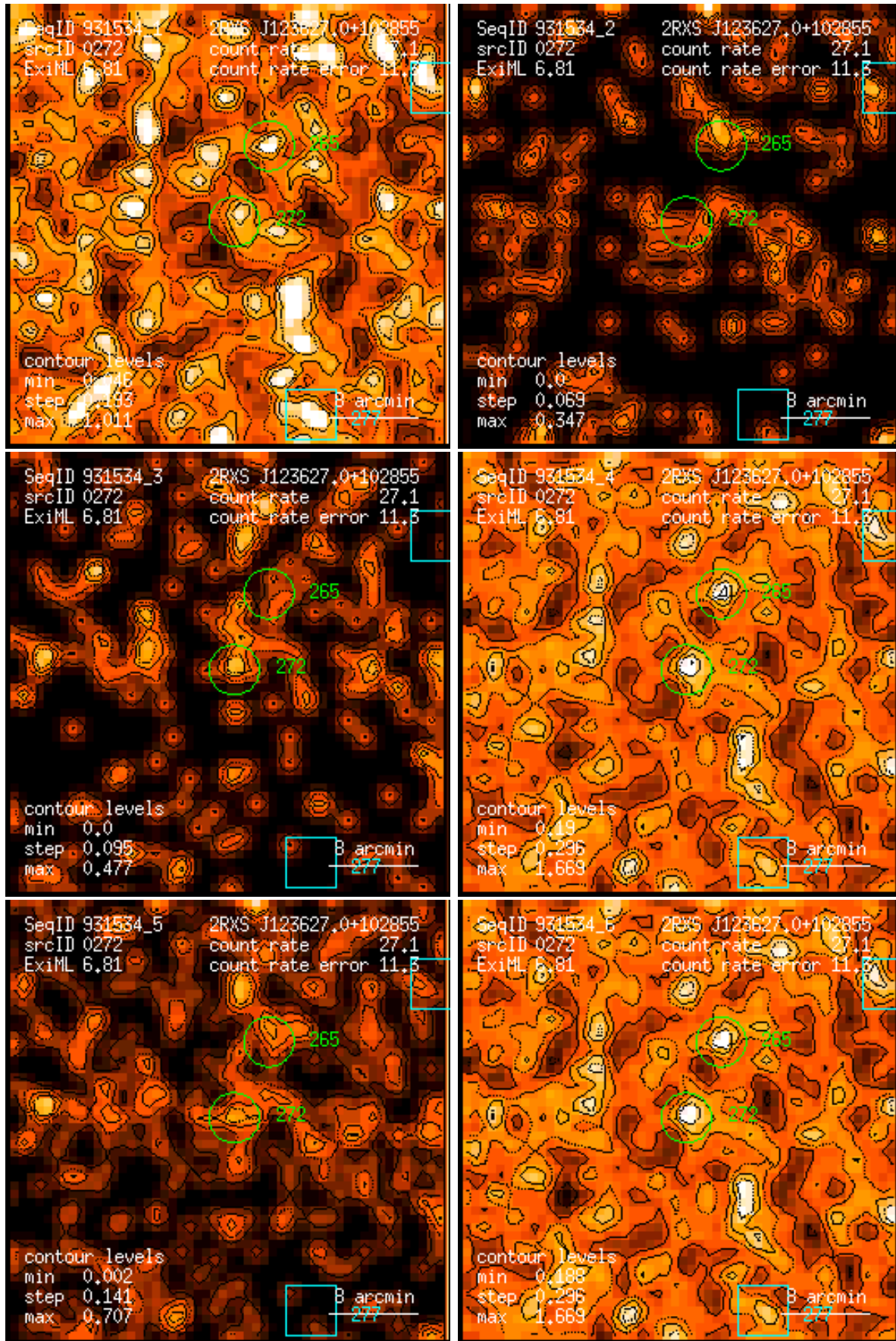
Figure 272: RASS 931534: detection 0272: band rate images, Gaussian filter: (1) PSPC channels 11 – 41, (2) 52 – 90, (3) 91 – 201, (4) 11 – 235, (5) 52 – 201, (6) 11 – 201. Broad band rates in counts/ks. Band rate contour levels in counts/ks/arcmin 2 .
