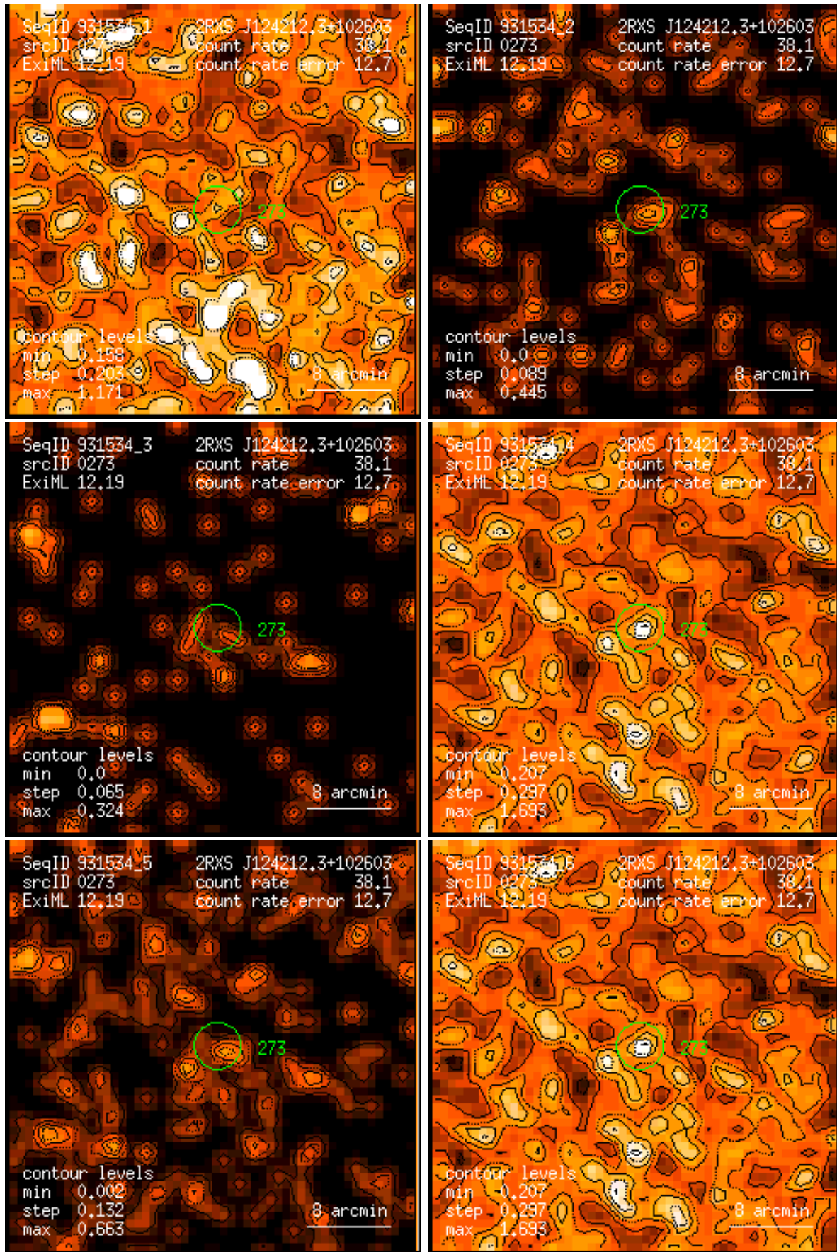
Figure 273: RASS 931534: detection 0273: band rate images, Gaussian filter: (1) PSPC channels 11 – 41, (2) 52 – 90, (3) 91 – 201, (4) 11 – 235, (5) 52 – 201, (6) 11 – 201. Broad band rates in counts/ks. Band rate contour levels in counts/ks/arcmin 2 .
