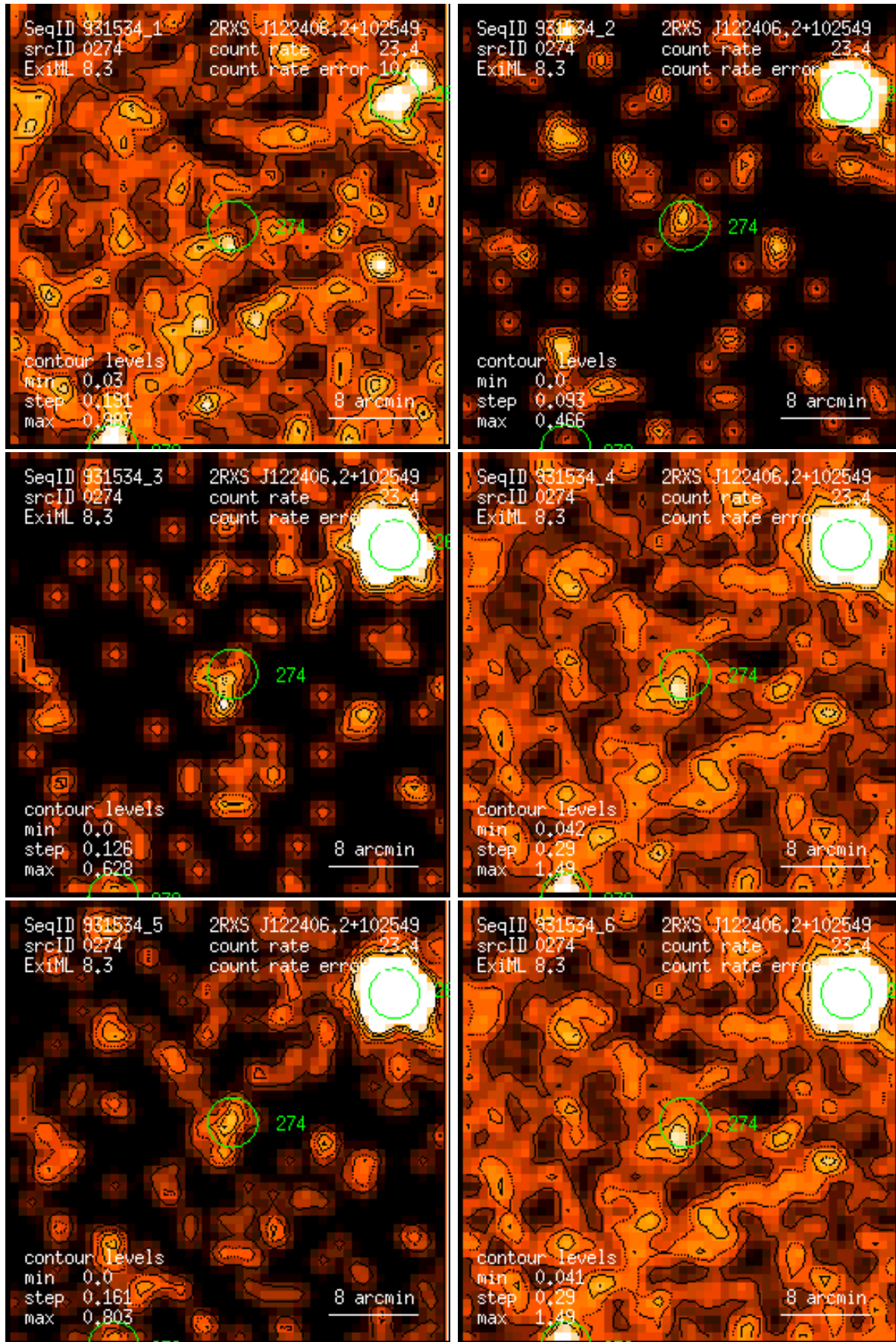
Figure 274: RASS 931534: detection 0274: band rate images, Gaussian filter: (1) PSPC channels 11 – 41, (2) 52 – 90, (3) 91 – 201, (4) 11 – 235, (5) 52 – 201, (6) 11 – 201. Broad band rates in counts/ks. Band rate contour levels in counts/ks/arcmin 2 .
