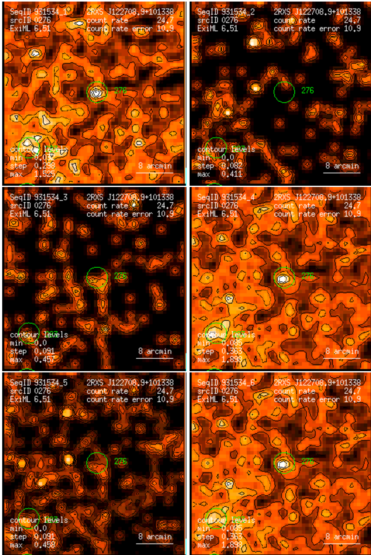
Figure 276: RASS 931534: detection 0276: band rate images, Gaussian filter: (1) PSPC channels 11 – 41, (2) 52 – 90, (3) 91 – 201, (4) 11 – 235, (5) 52 – 201, (6) 11 – 201. Broad band rates in counts/ks. Band rate contour levels in counts/ks/arcmin 2 .
