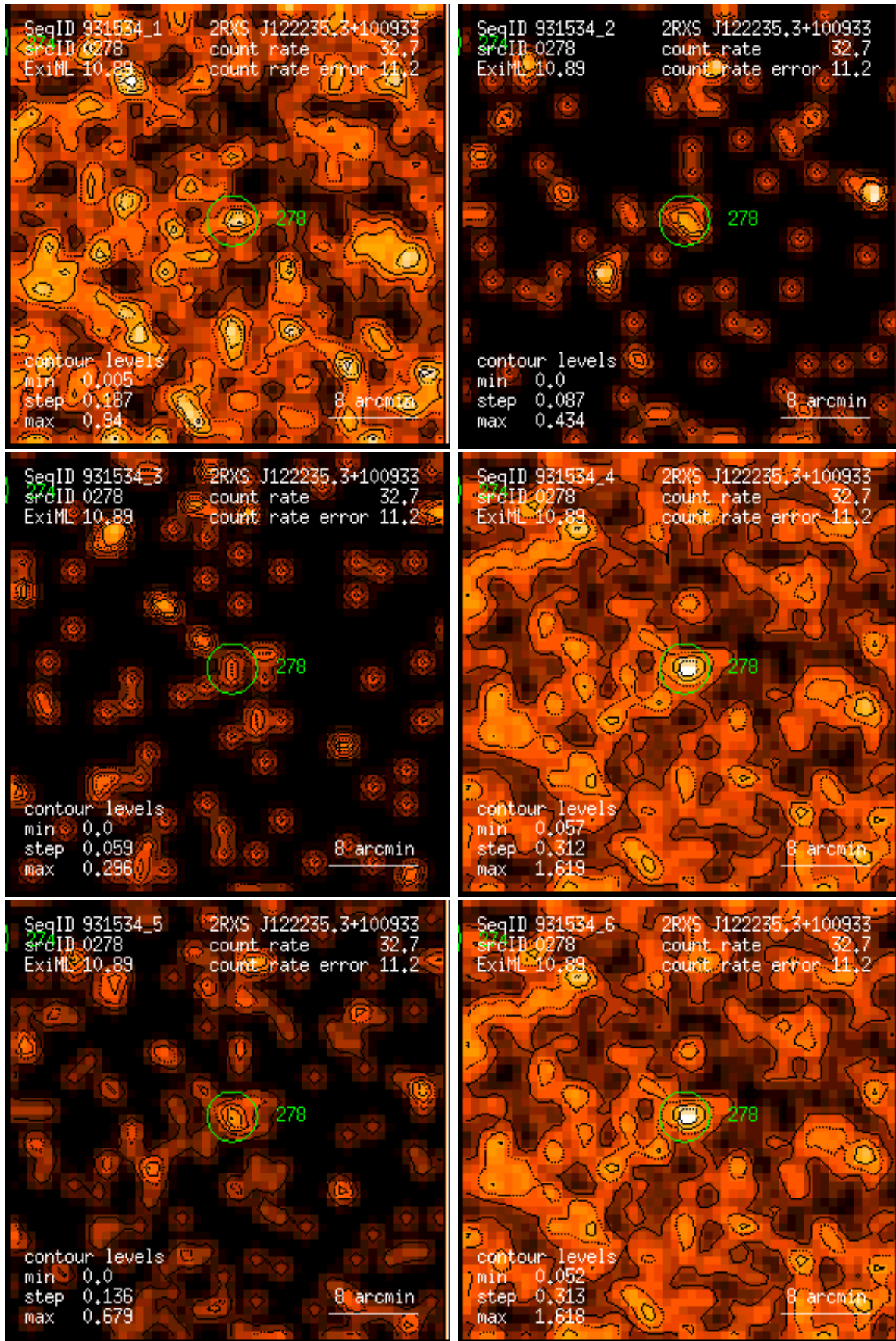
Figure 278: RASS 931534: detection 0278: band rate images, Gaussian filter: (1) PSPC channels 11 – 41, (2) 52 – 90, (3) 91 – 201, (4) 11 – 235, (5) 52 – 201, (6) 11 – 201. Broad band rates in counts/ks. Band rate contour levels in counts/ks/arcmin 2 .
