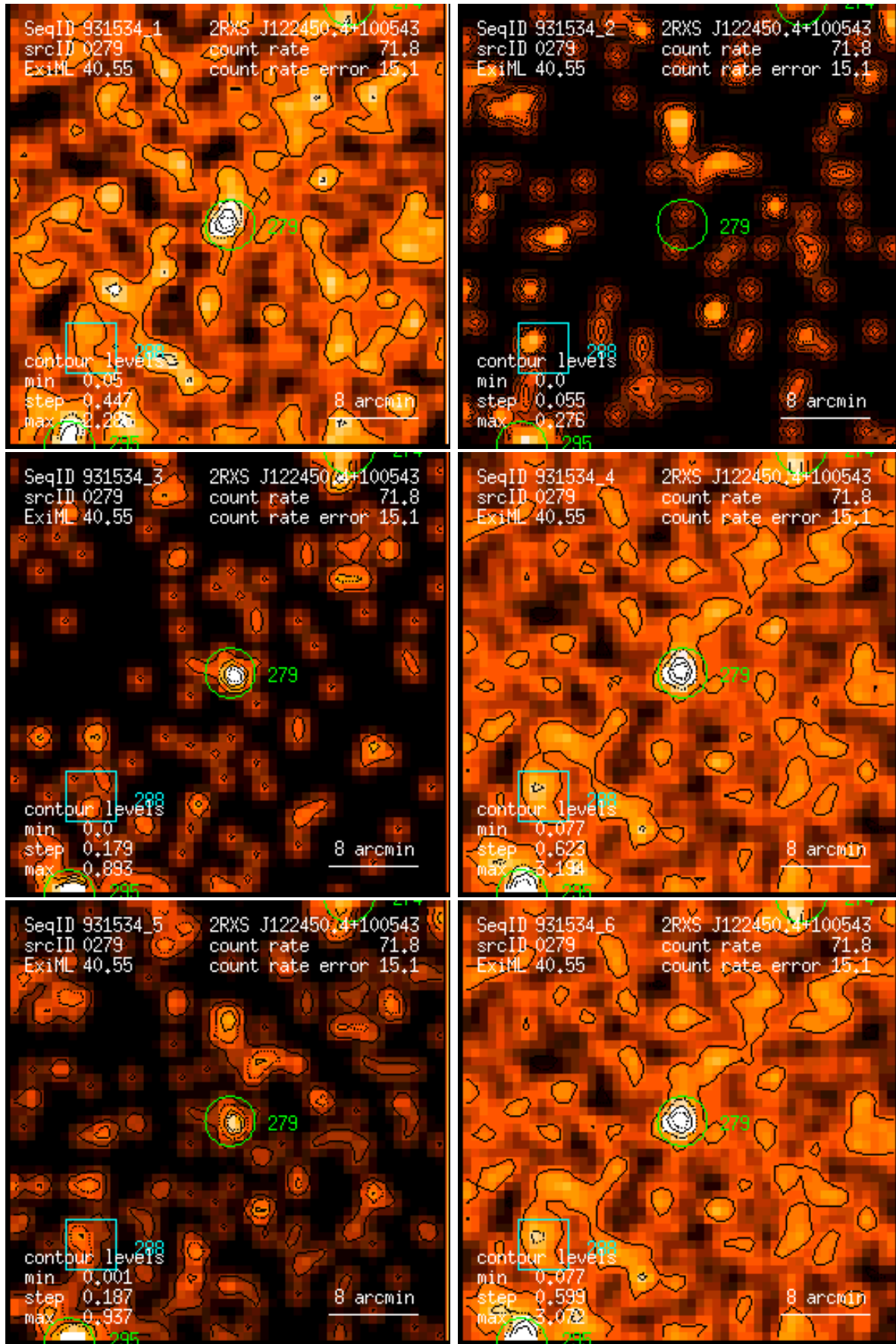
Figure 279: RASS 931534: detection 0279: band rate images, Gaussian filter: (1) PSPC channels 11 – 41, (2) 52 – 90, (3) 91 – 201, (4) 11 – 235, (5) 52 – 201, (6) 11 – 201. Broad band rates in counts/ks. Band rate contour levels in counts/ks/arcmin 2 .
