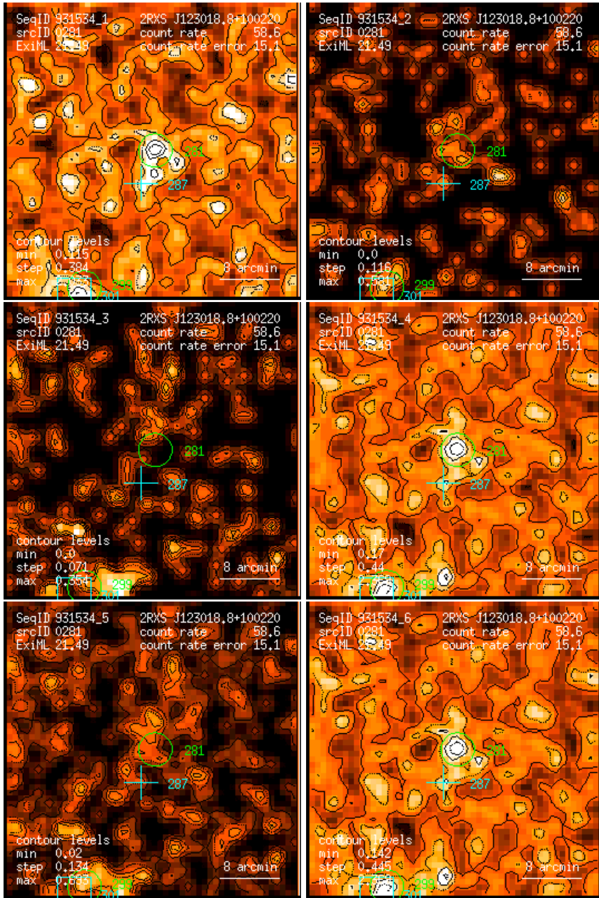
Figure 281: RASS 931534: detection 0281: band rate images, Gaussian filter: (1) PSPC channels 11 – 41, (2) 52 – 90, (3) 91 – 201, (4) 11 – 235, (5) 52 – 201, (6) 11 – 201. Broad band rates in counts/ks. Band rate contour levels in counts/ks/arcmin 2 .
