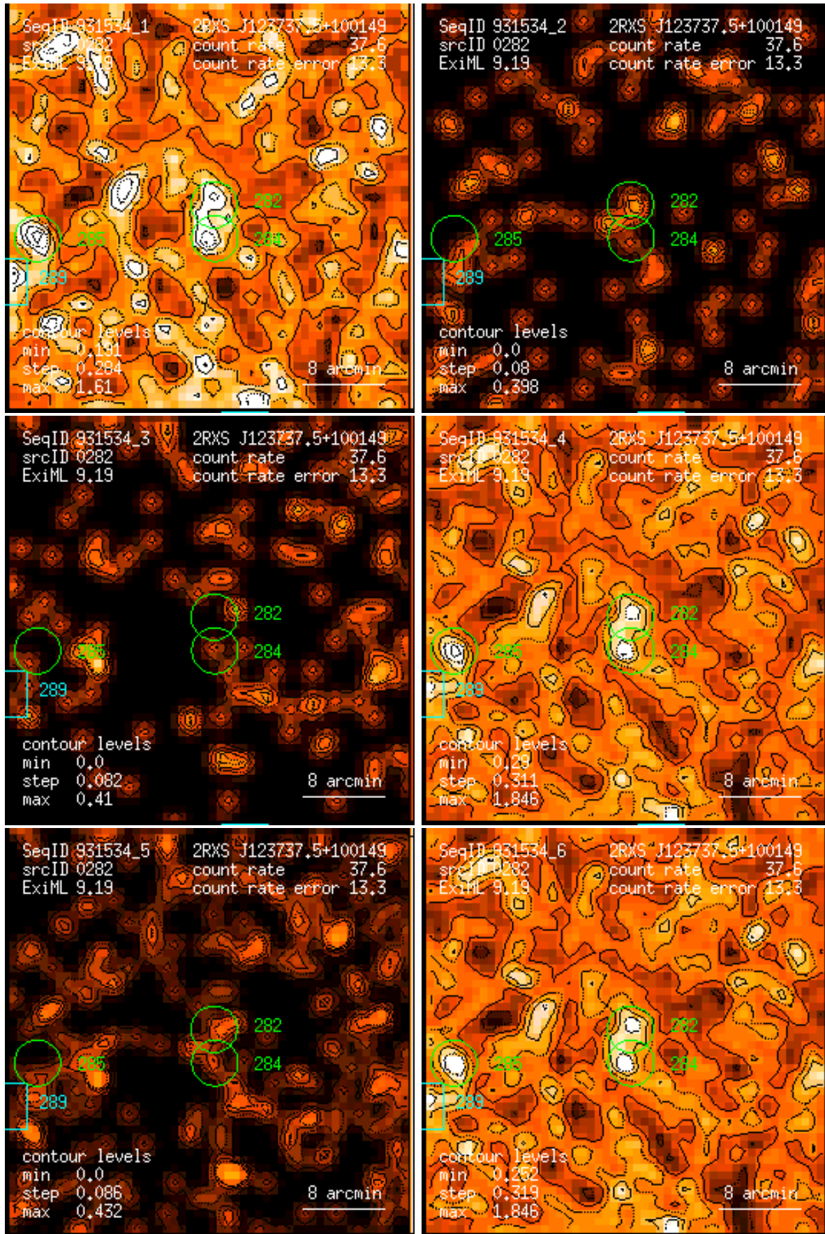
Figure 282: RASS 931534: detection 0282: band rate images, Gaussian filter: (1) PSPC channels 11 – 41, (2) 52 – 90, (3) 91 – 201, (4) 11 – 235, (5) 52 – 201, (6) 11 – 201. Broad band rates in counts/ks. Band rate contour levels in counts/ks/arcmin 2 .
