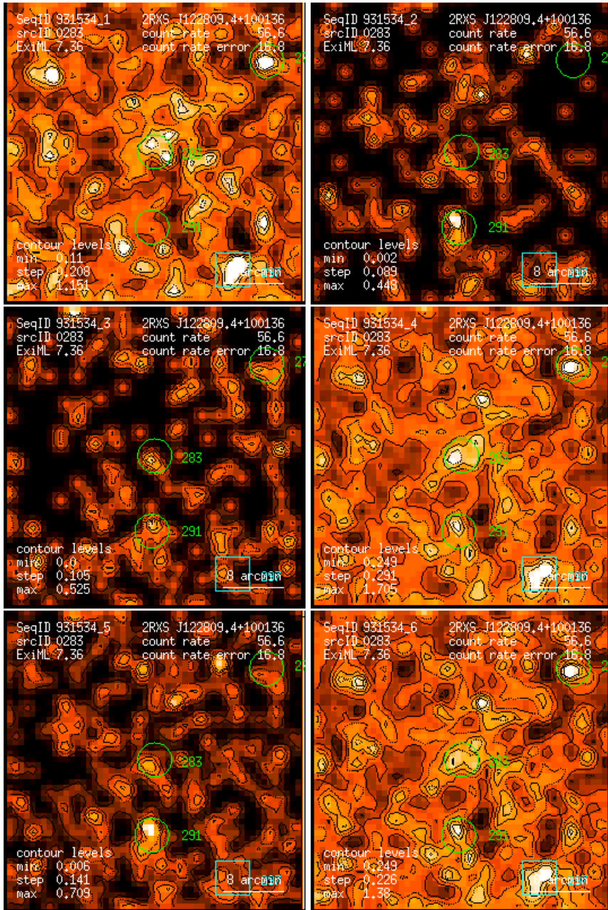
Figure 283: RASS 931534: detection 0283: band rate images, Gaussian filter: (1) PSPC channels 11 – 41, (2) 52 – 90, (3) 91 – 201, (4) 11 – 235, (5) 52 – 201, (6) 11 – 201. Broad band rates in counts/ks. Band rate contour levels in counts/ks/arcmin 2 .
