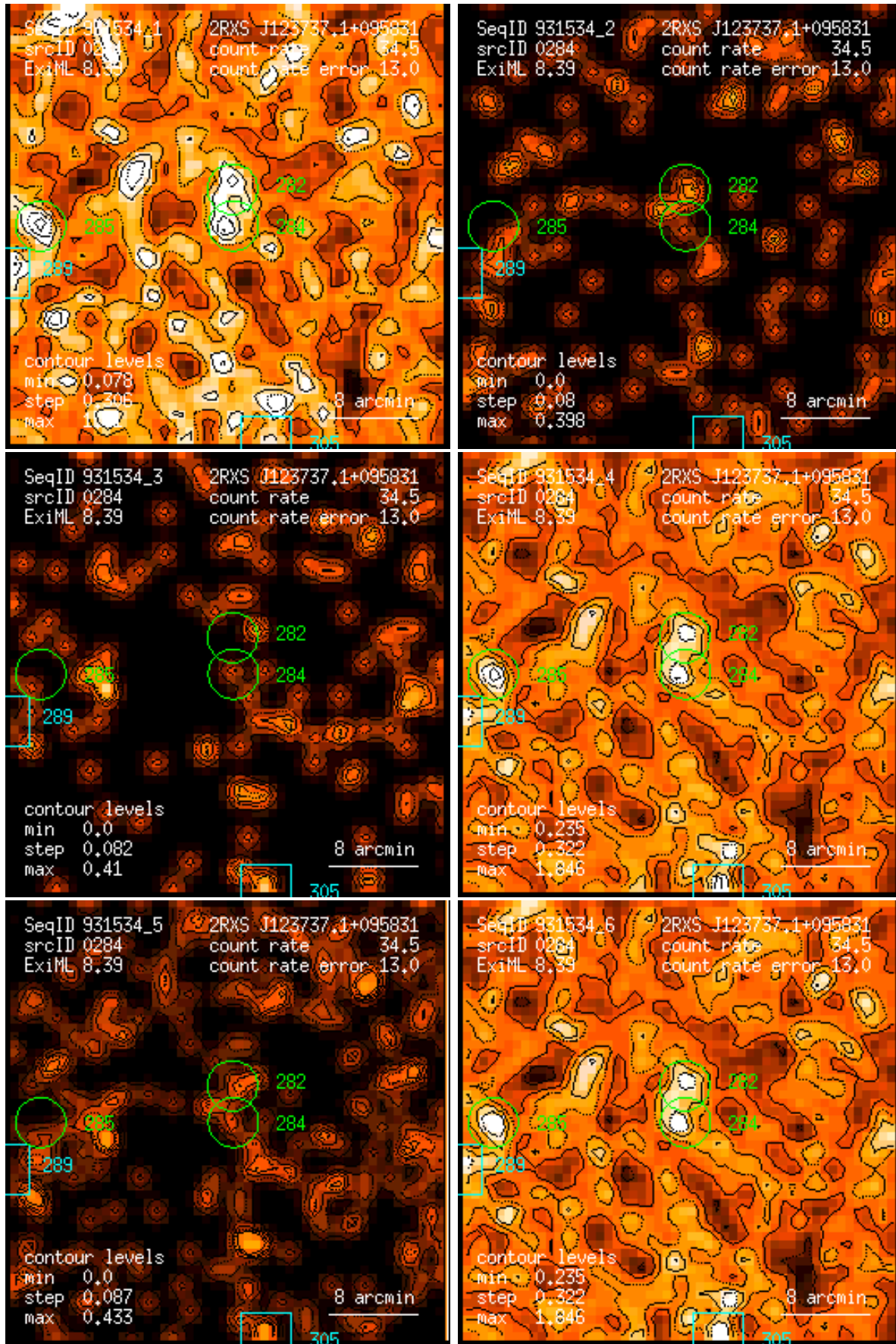
Figure 284: RASS 931534: detection 0284: band rate images, Gaussian filter: (1) PSPC channels 11 – 41, (2) 52 – 90, (3) 91 – 201, (4) 11 – 235, (5) 52 – 201, (6) 11 – 201. Broad band rates in counts/ks. Band rate contour levels in counts/ks/arcmin 2 .
