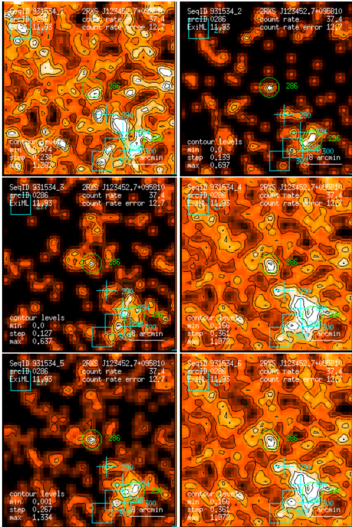
Figure 286: RASS 931534: detection 0286: band rate images, Gaussian filter: (1) PSPC channels 11 – 41, (2) 52 – 90, (3) 91 – 201, (4) 11 – 235, (5) 52 – 201, (6) 11 – 201. Broad band rates in counts/ks. Band rate contour levels in counts/ks/arcmin 2 .
