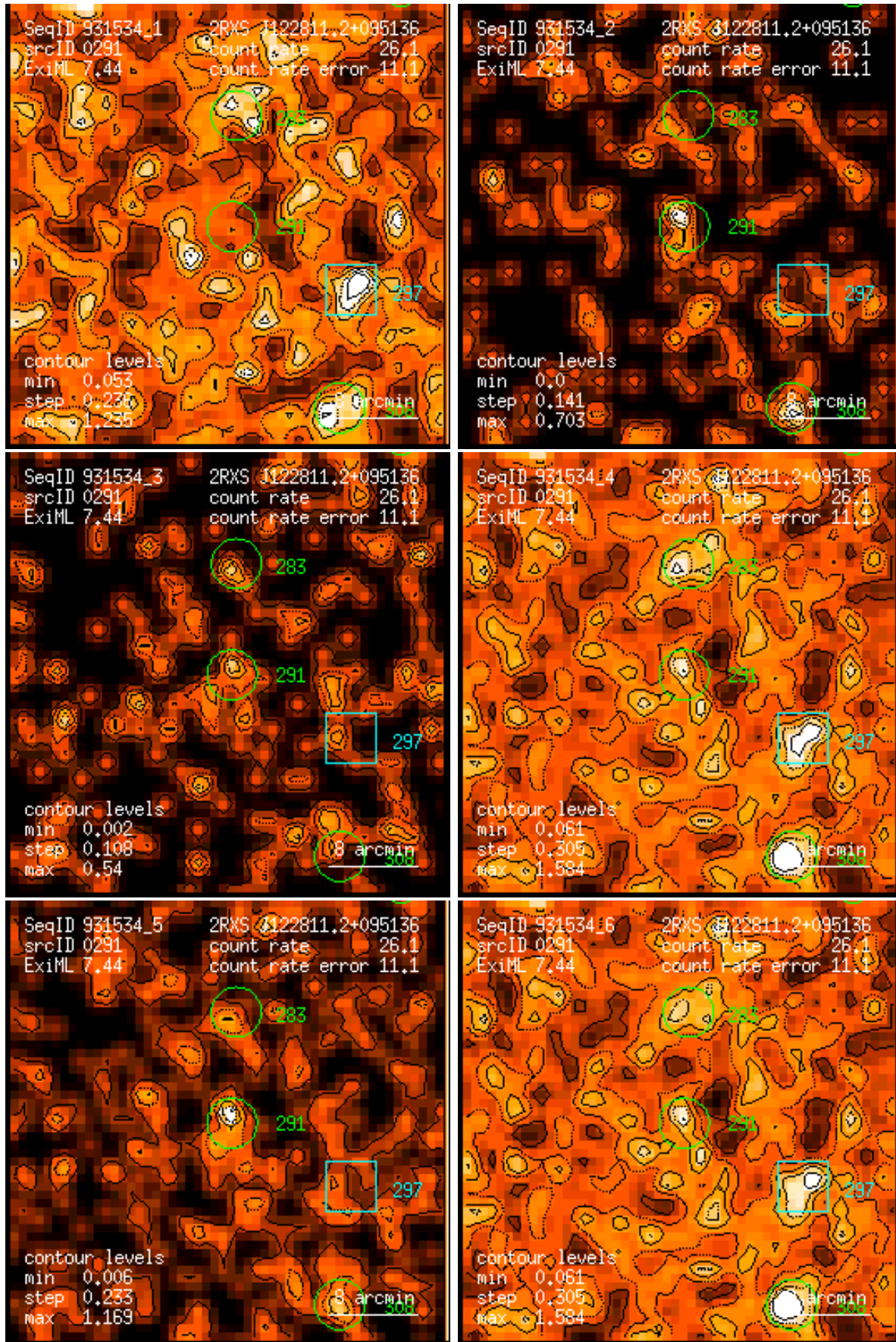
Figure 291: RASS 931534: detection 0291: band rate images, Gaussian filter: (1) PSPC channels 11 – 41, (2) 52 – 90, (3) 91 – 201, (4) 11 – 235, (5) 52 – 201, (6) 11 – 201. Broad band rates in counts/ks. Band rate contour levels in counts/ks/arcmin 2 .
