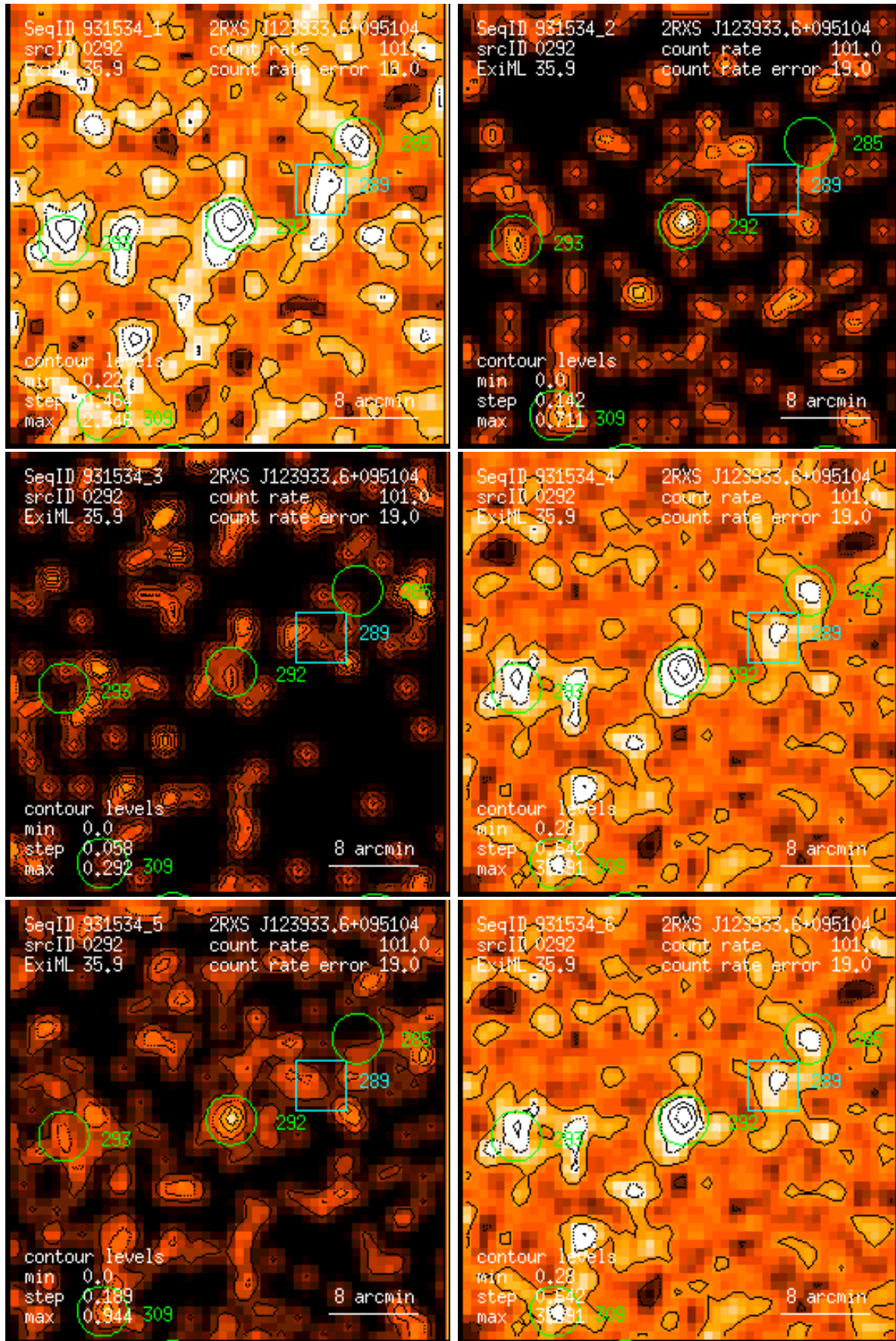
Figure 292: RASS 931534: detection 0292: band rate images, Gaussian filter: (1) PSPC channels 11 – 41, (2) 52 – 90, (3) 91 – 201, (4) 11 – 235, (5) 52 – 201, (6) 11 – 201. Broad band rates in counts/ks. Band rate contour levels in counts/ks/arcmin 2 .
