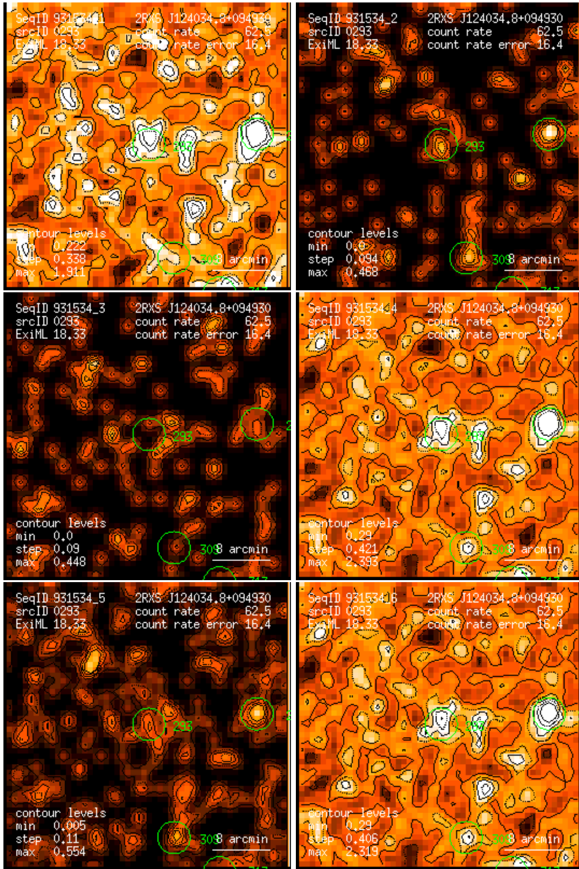
Figure 293: RASS 931534: detection 0293: band rate images, Gaussian filter: (1) PSPC channels 11 – 41, (2) 52 – 90, (3) 91 – 201, (4) 11 – 235, (5) 52 – 201, (6) 11 – 201. Broad band rates in counts/ks. Band rate contour levels in counts/ks/arcmin 2 .
