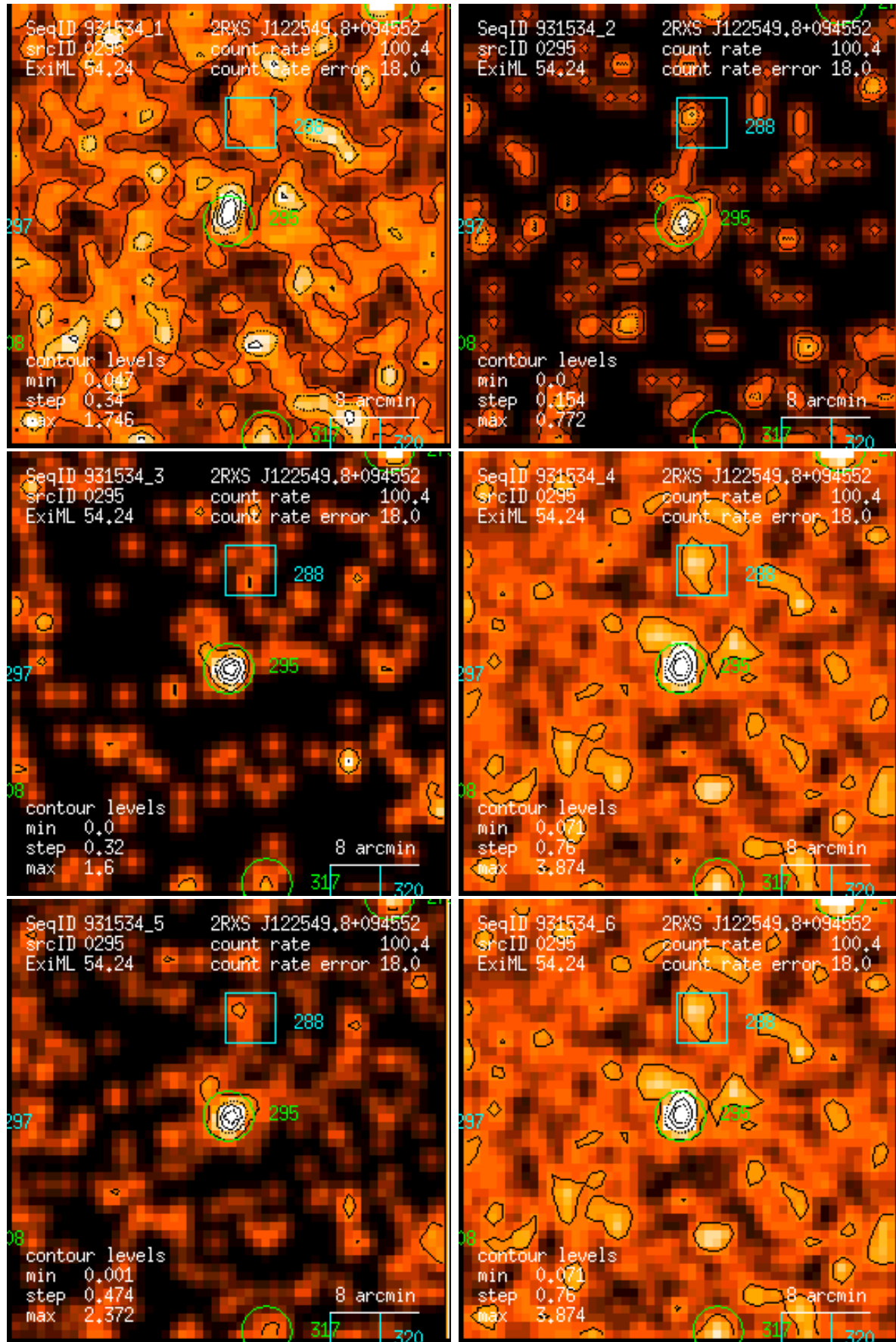
Figure 295: RASS 931534: detection 0295: band rate images, Gaussian filter: (1) PSPC channels 11 – 41, (2) 52 – 90, (3) 91 – 201, (4) 11 – 235, (5) 52 – 201, (6) 11 – 201. Broad band rates in counts/ks. Band rate contour levels in counts/ks/arcmin 2 .
