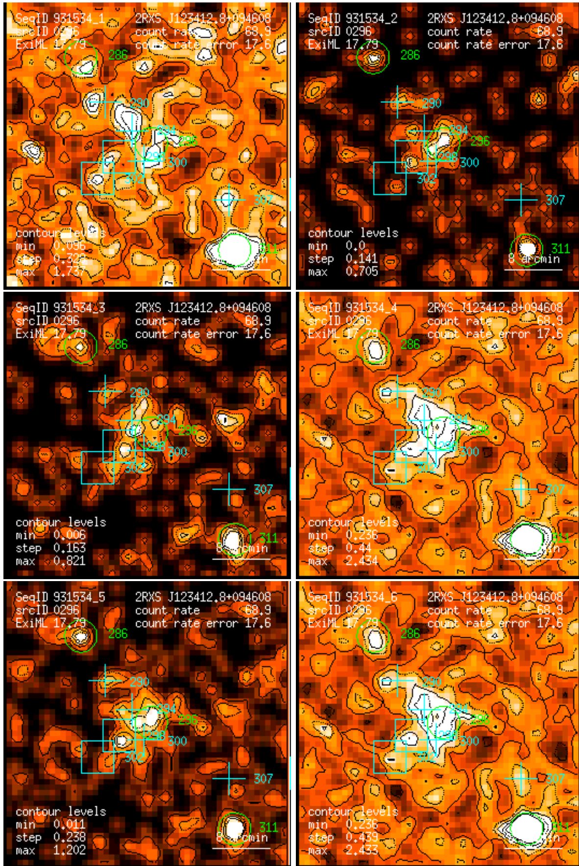
Figure 296: RASS 931534: detection 0296: band rate images, Gaussian filter: (1) PSPC channels 11 – 41, (2) 52 – 90, (3) 91 – 201, (4) 11 – 235, (5) 52 – 201, (6) 11 – 201. Broad band rates in counts/ks. Band rate contour levels in counts/ks/arcmin 2 .
