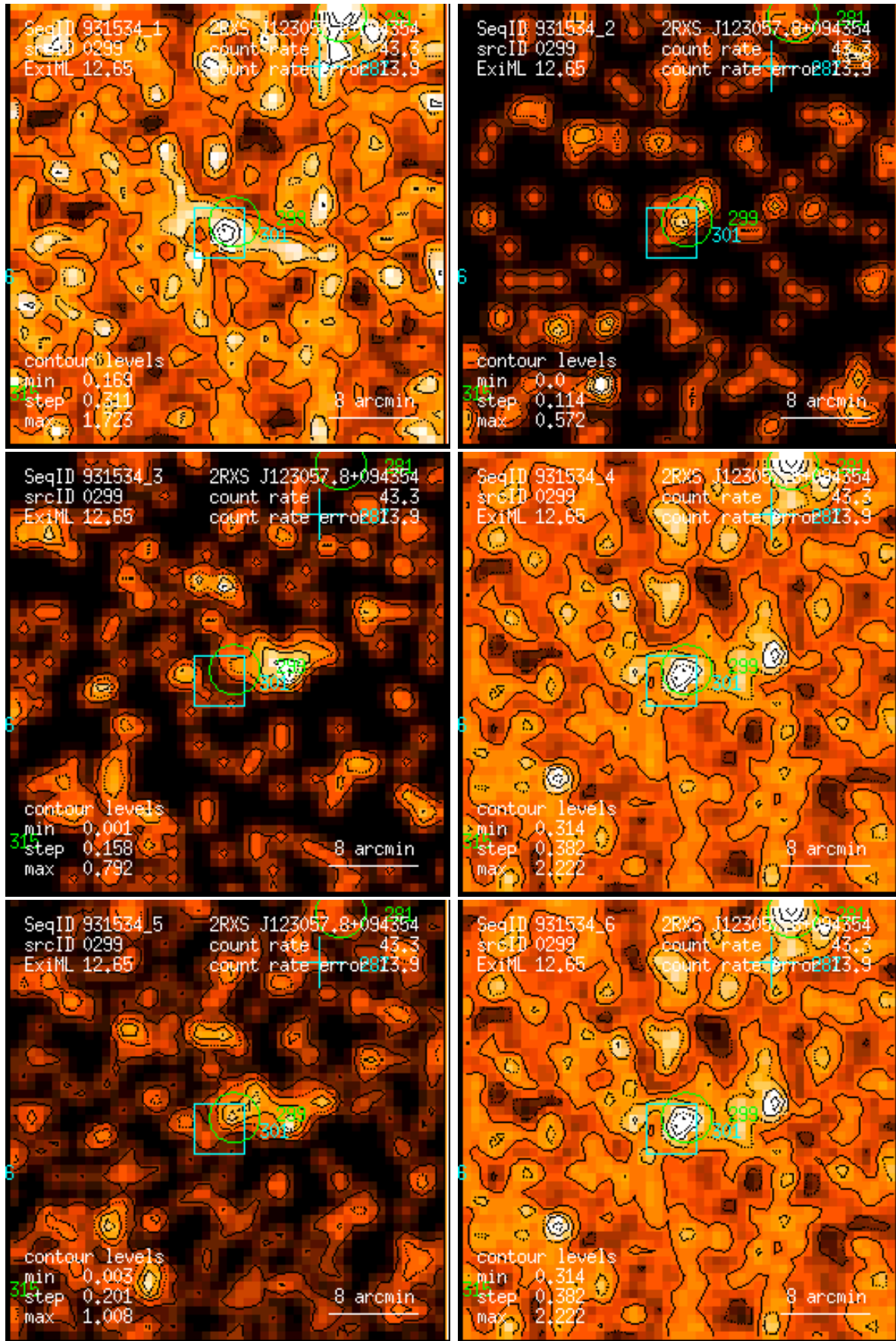
Figure 299: RASS 931534: detection 0299: band rate images, Gaussian filter: (1) PSPC channels 11 – 41, (2) 52 – 90, (3) 91 – 201, (4) 11 – 235, (5) 52 – 201, (6) 11 – 201. Broad band rates in counts/ks. Band rate contour levels in counts/ks/arcmin 2 .
