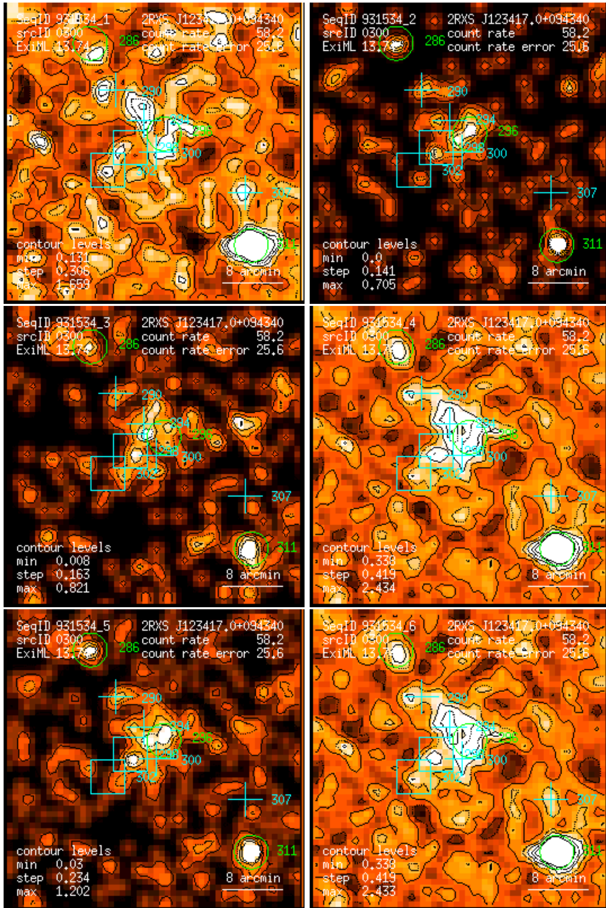
Figure 300: RASS 931534: detection 0300: band rate images, Gaussian filter: (1) PSPC channels 11 – 41, (2) 52 – 90, (3) 91 – 201, (4) 11 – 235, (5) 52 – 201, (6) 11 – 201. Broad band rates in counts/ks. Band rate contour levels in counts/ks/arcmin 2 .
