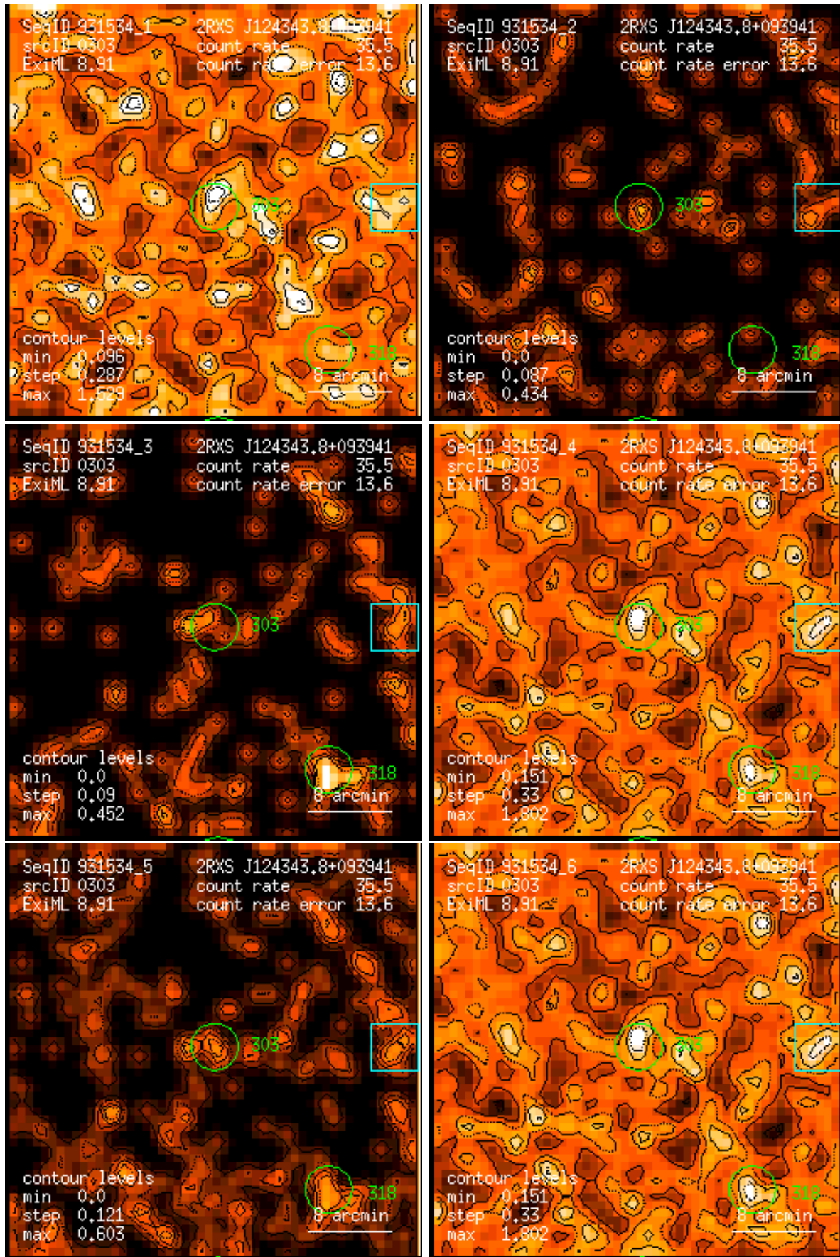
Figure 303: RASS 931534: detection 0303: band rate images, Gaussian filter: (1) PSPC channels 11 – 41, (2) 52 – 90, (3) 91 – 201, (4) 11 – 235, (5) 52 – 201, (6) 11 – 201. Broad band rates in counts/ks. Band rate contour levels in counts/ks/arcmin 2 .
