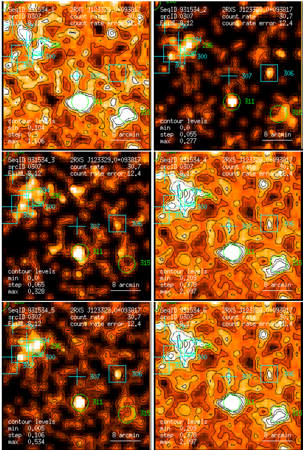
Figure 307: RASS 931534: detection 0307: band rate images, Gaussian filter: (1) PSPC channels 11 – 41, (2) 52 – 90, (3) 91 – 201, (4) 11 – 235, (5) 52 – 201, (6) 11 – 201. Broad band rates in counts/ks. Band rate contour levels in counts/ks/arcmin 2 .
