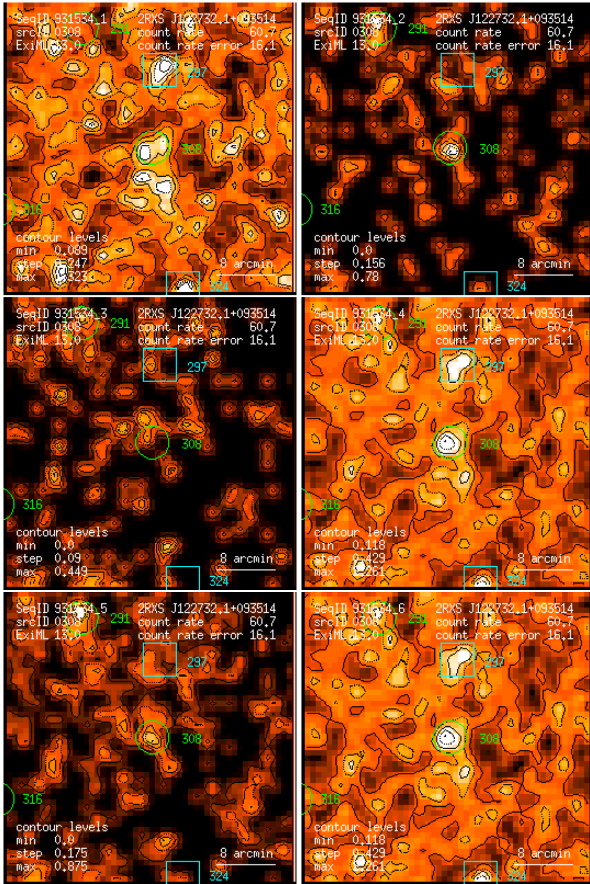
Figure 308: RASS 931534: detection 0308: band rate images, Gaussian filter: (1) PSPC channels 11 – 41, (2) 52 – 90, (3) 91 – 201, (4) 11 – 235, (5) 52 – 201, (6) 11 – 201. Broad band rates in counts/ks. Band rate contour levels in counts/ks/arcmin 2 .
