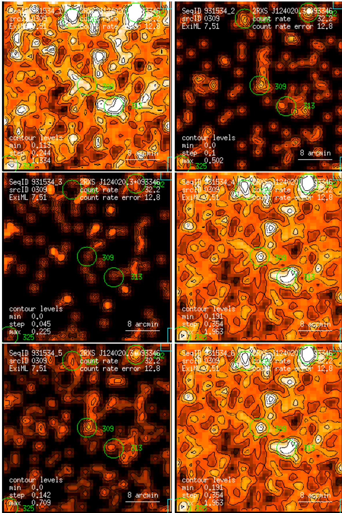
Figure 309: RASS 931534: detection 0309: band rate images, Gaussian filter: (1) PSPC channels 11 – 41, (2) 52 – 90, (3) 91 – 201, (4) 11 – 235, (5) 52 – 201, (6) 11 – 201. Broad band rates in counts/ks. Band rate contour levels in counts/ks/arcmin 2 .
