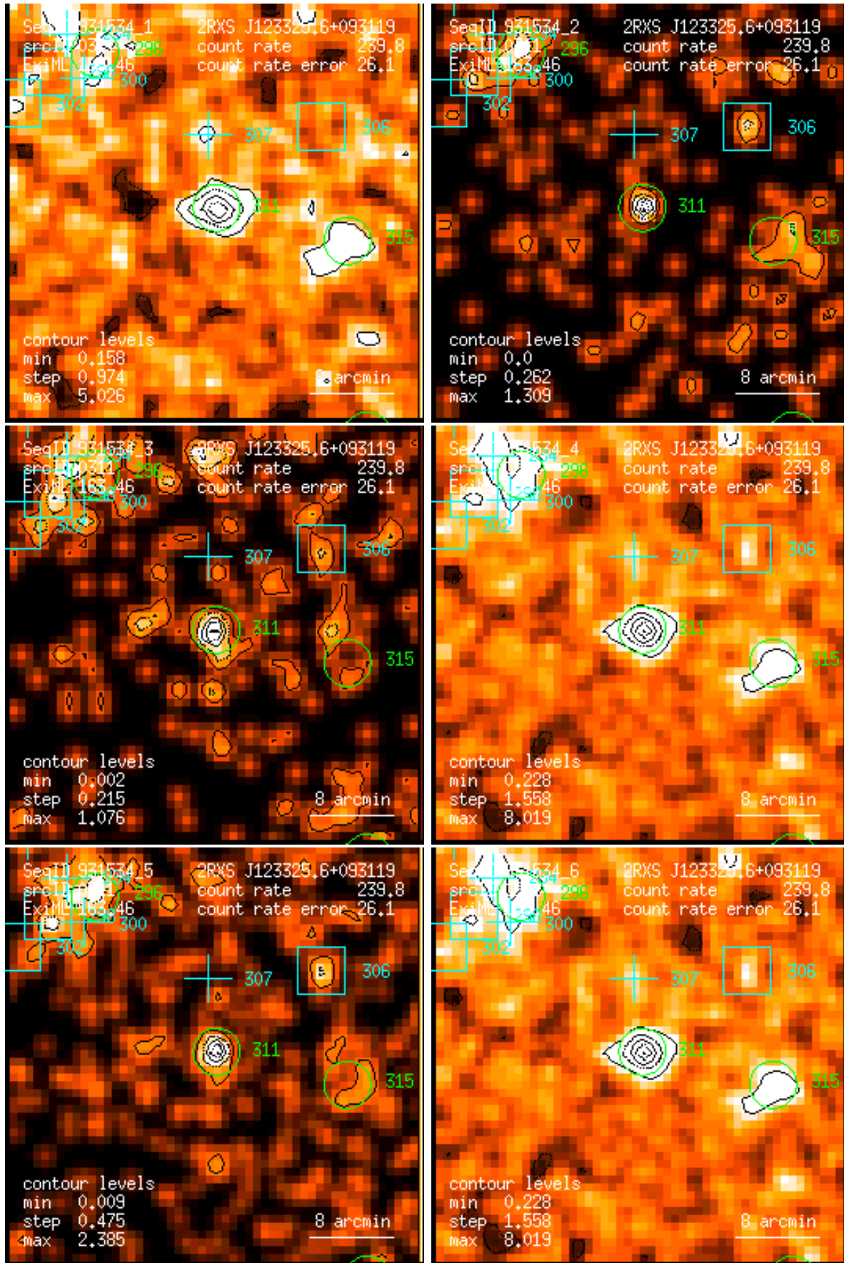
Figure 311: RASS 931534: detection 0311: band rate images, Gaussian filter: (1) PSPC channels 11 – 41, (2) 52 – 90, (3) 91 – 201, (4) 11 – 235, (5) 52 – 201, (6) 11 – 201. Broad band rates in counts/ks. Band rate contour levels in counts/ks/arcmin 2 .
