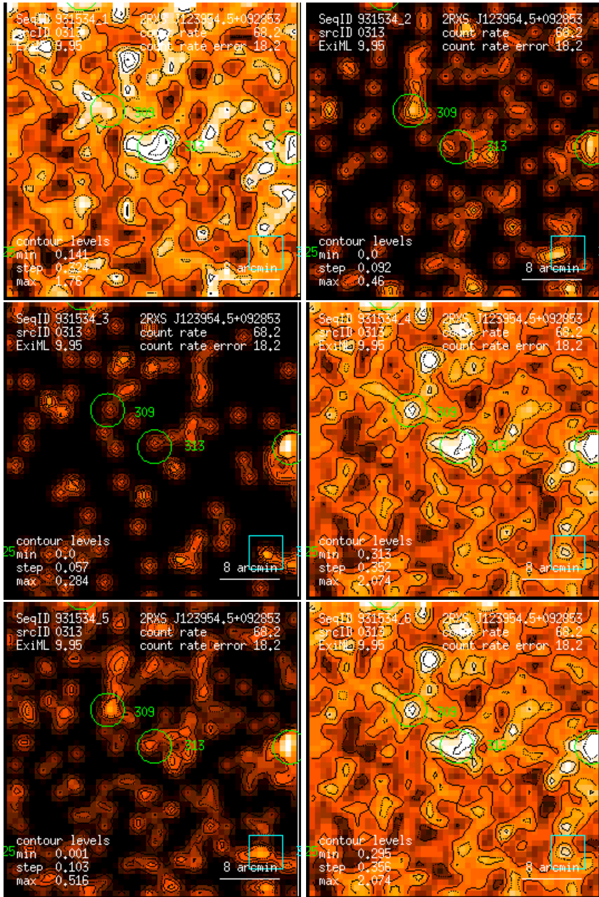
Figure 313: RASS 931534: detection 0313: band rate images, Gaussian filter: (1) PSPC channels 11 – 41, (2) 52 – 90, (3) 91 – 201, (4) 11 – 235, (5) 52 – 201, (6) 11 – 201. Broad band rates in counts/ks. Band rate contour levels in counts/ks/arcmin 2 .
