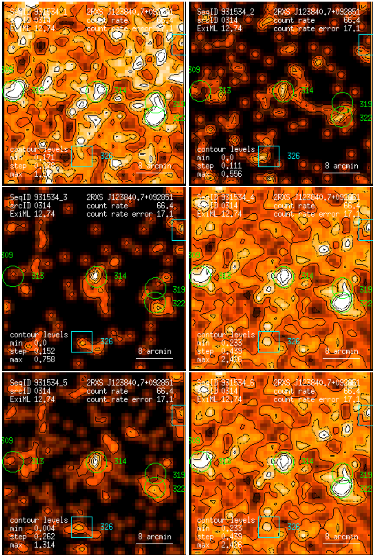
Figure 314: RASS 931534: detection 0314: band rate images, Gaussian filter: (1) PSPC channels 11 – 41, (2) 52 – 90, (3) 91 – 201, (4) 11 – 235, (5) 52 – 201, (6) 11 – 201. Broad band rates in counts/ks. Band rate contour levels in counts/ks/arcmin 2 .
