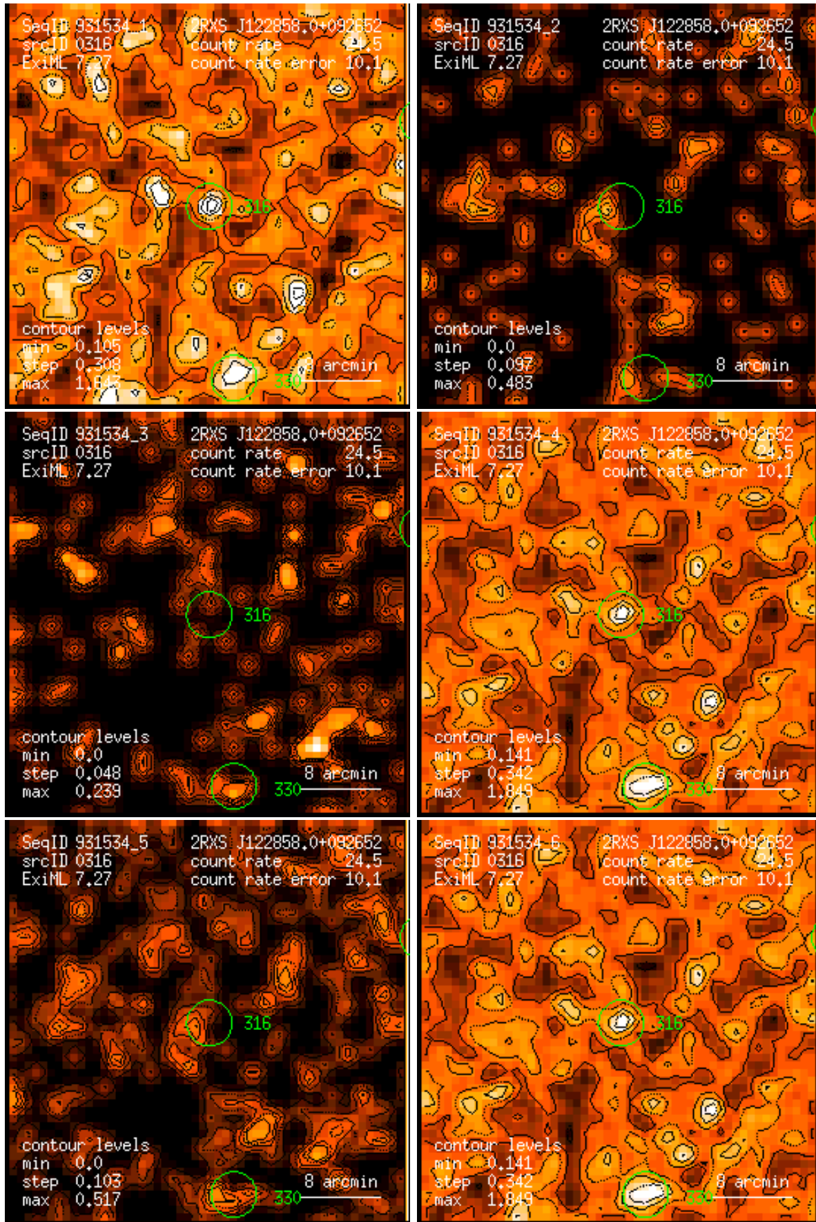
Figure 316: RASS 931534: detection 0316: band rate images, Gaussian filter: (1) PSPC channels 11 – 41, (2) 52 – 90, (3) 91 – 201, (4) 11 – 235, (5) 52 – 201, (6) 11 – 201. Broad band rates in counts/ks. Band rate contour levels in counts/ks/arcmin 2 .
