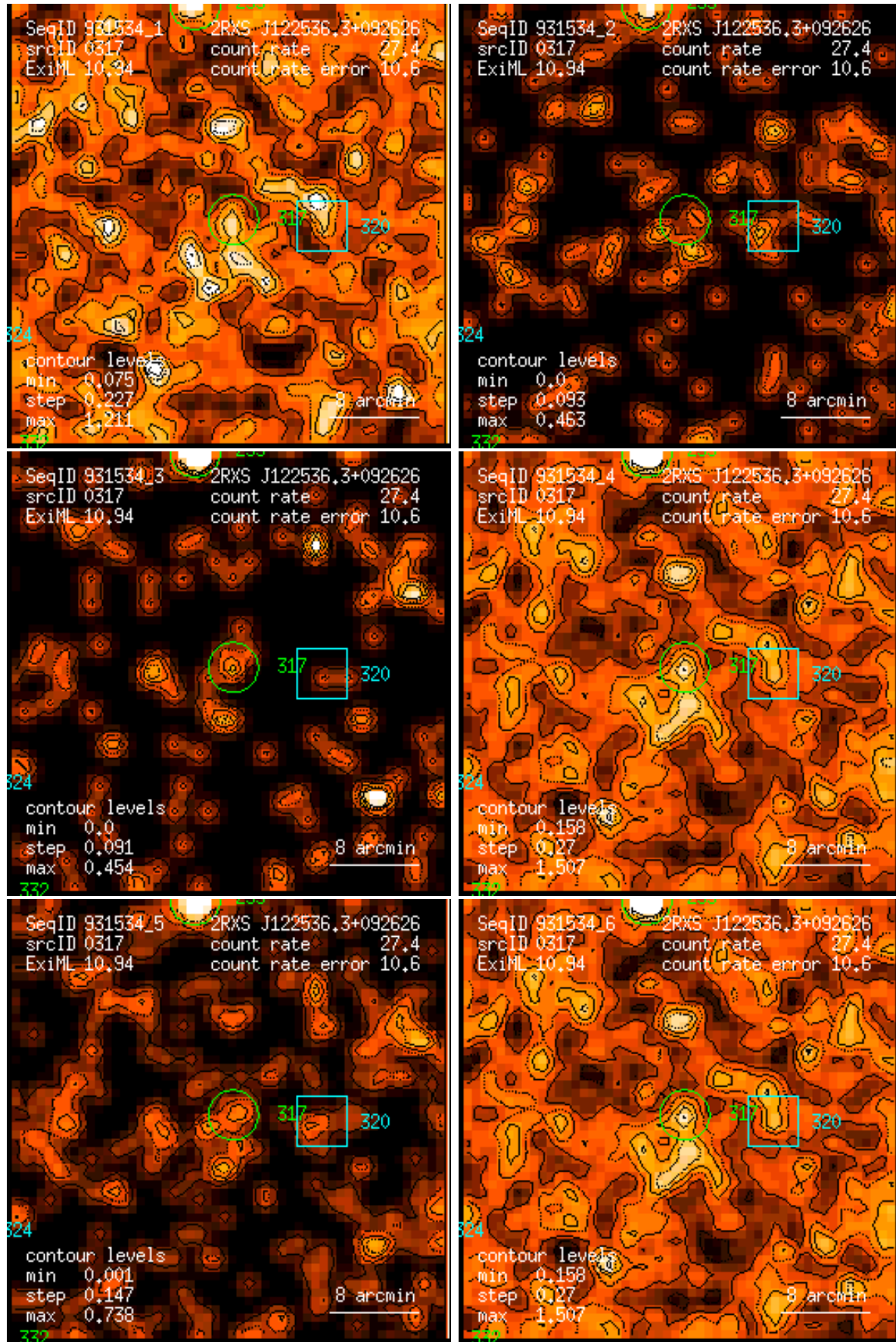
Figure 317: RASS 931534: detection 0317: band rate images, Gaussian filter: (1) PSPC channels 11 – 41, (2) 52 – 90, (3) 91 – 201, (4) 11 – 235, (5) 52 – 201, (6) 11 – 201. Broad band rates in counts/ks. Band rate contour levels in counts/ks/arcmin 2 .
