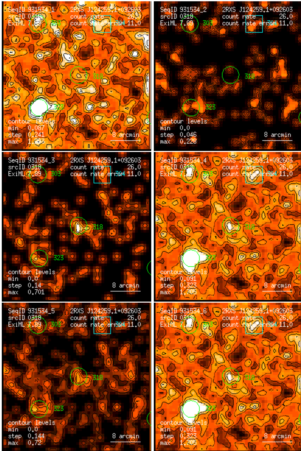
Figure 318: RASS 931534: detection 0318: band rate images, Gaussian filter: (1) PSPC channels 11 – 41, (2) 52 – 90, (3) 91 – 201, (4) 11 – 235, (5) 52 – 201, (6) 11 – 201. Broad band rates in counts/ks. Band rate contour levels in counts/ks/arcmin 2 .
