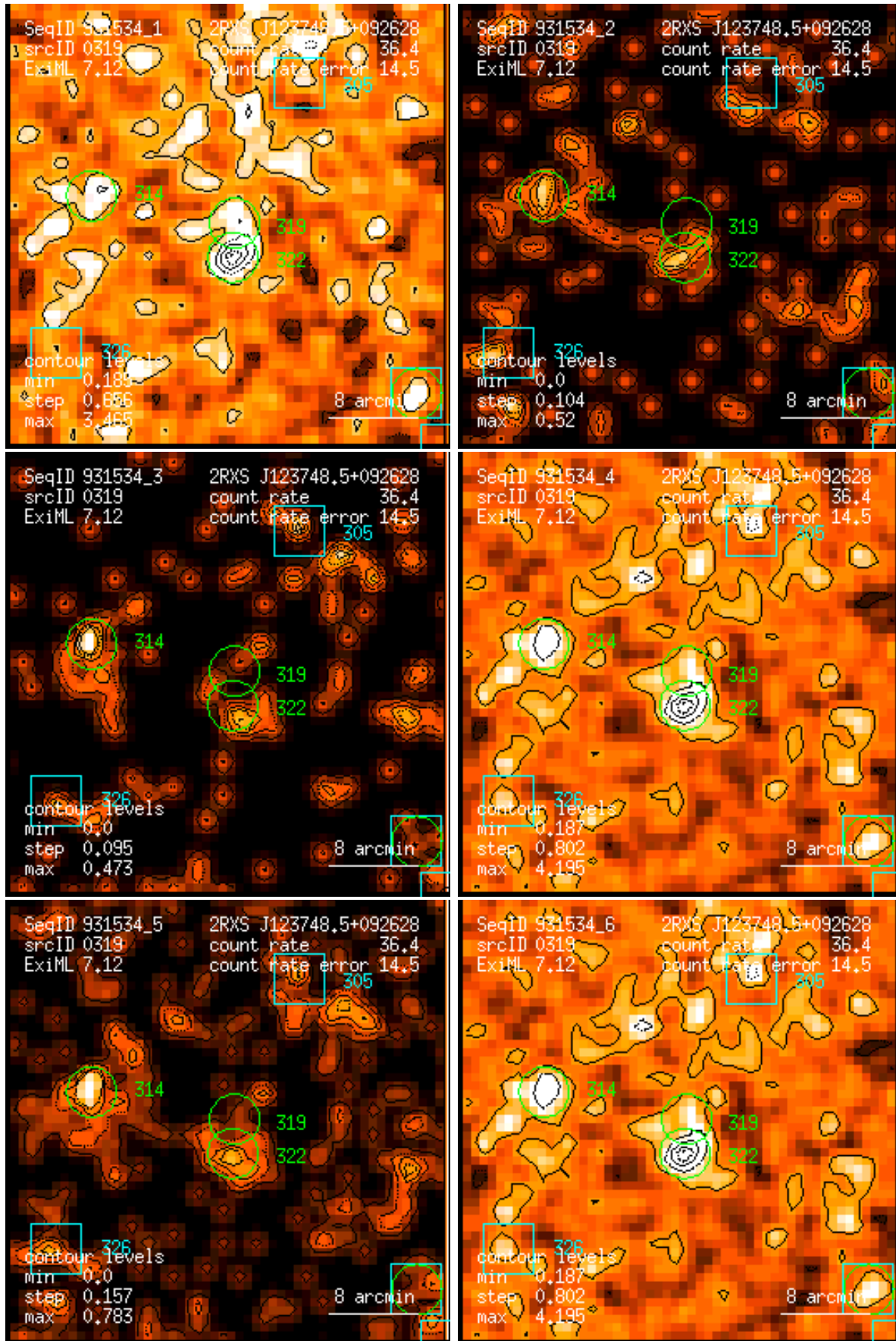
Figure 319: RASS 931534: detection 0319: band rate images, Gaussian filter: (1) PSPC channels 11 – 41, (2) 52 – 90, (3) 91 – 201, (4) 11 – 235, (5) 52 – 201, (6) 11 – 201. Broad band rates in counts/ks. Band rate contour levels in counts/ks/arcmin 2 .
