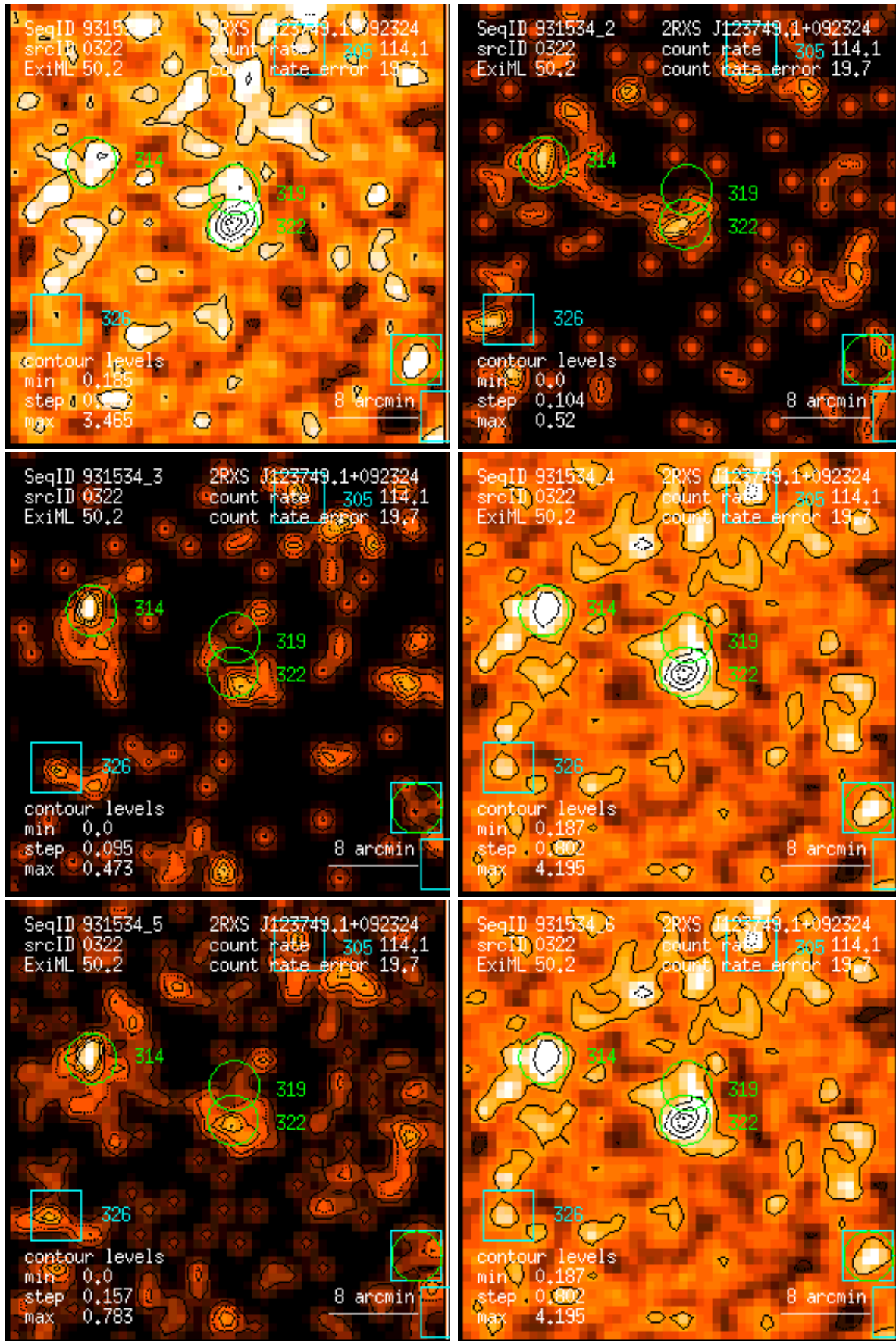
Figure 322: RASS 931534: detection 0322: band rate images, Gaussian filter: (1) PSPC channels 11 – 41, (2) 52 – 90, (3) 91 – 201, (4) 11 – 235, (5) 52 – 201, (6) 11 – 201. Broad band rates in counts/ks. Band rate contour levels in counts/ks/arcmin 2 .
