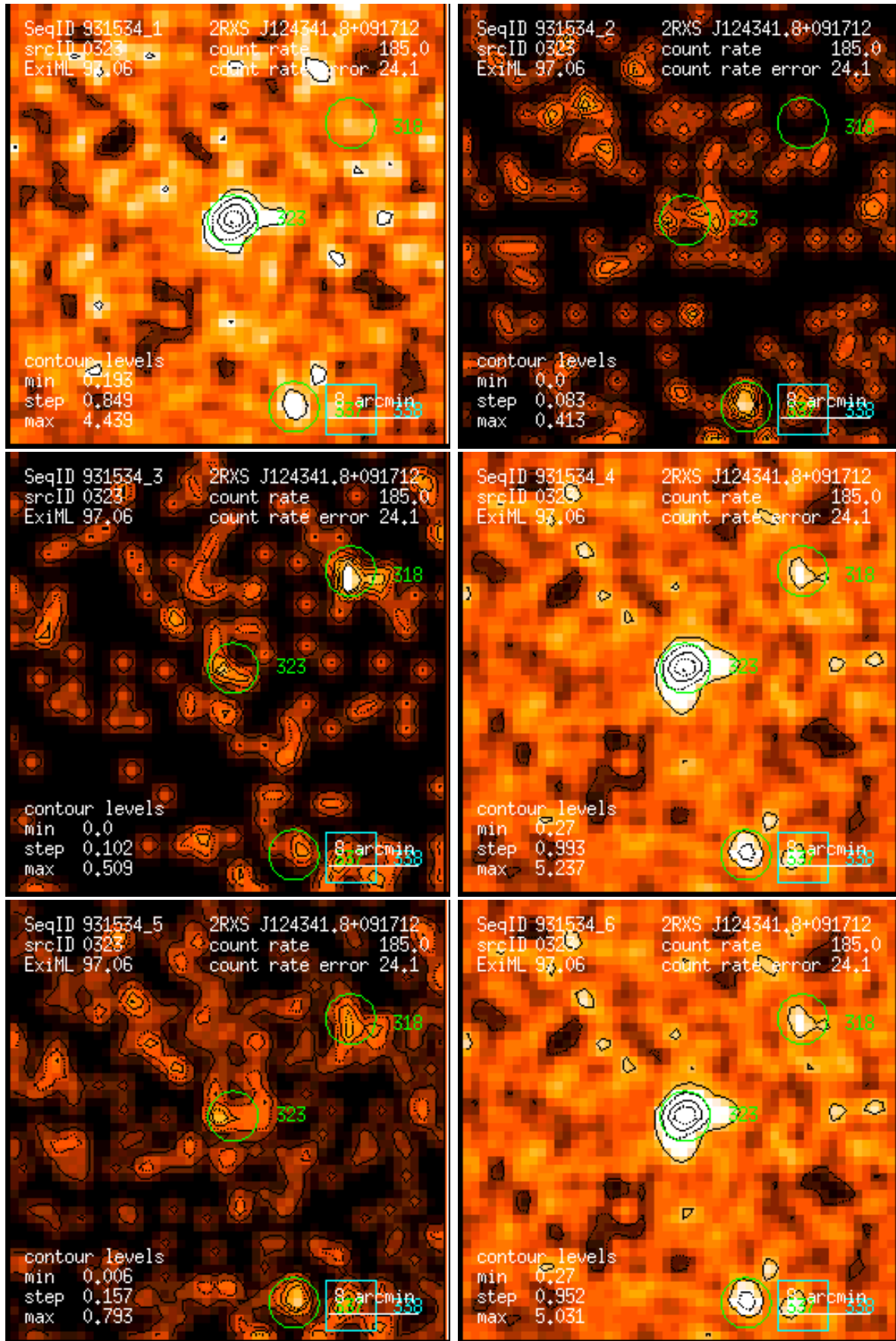
Figure 323: RASS 931534: detection 0323: band rate images, Gaussian filter: (1) PSPC channels 11 – 41, (2) 52 – 90, (3) 91 – 201, (4) 11 – 235, (5) 52 – 201, (6) 11 – 201. Broad band rates in counts/ks. Band rate contour levels in counts/ks/arcmin 2 .
