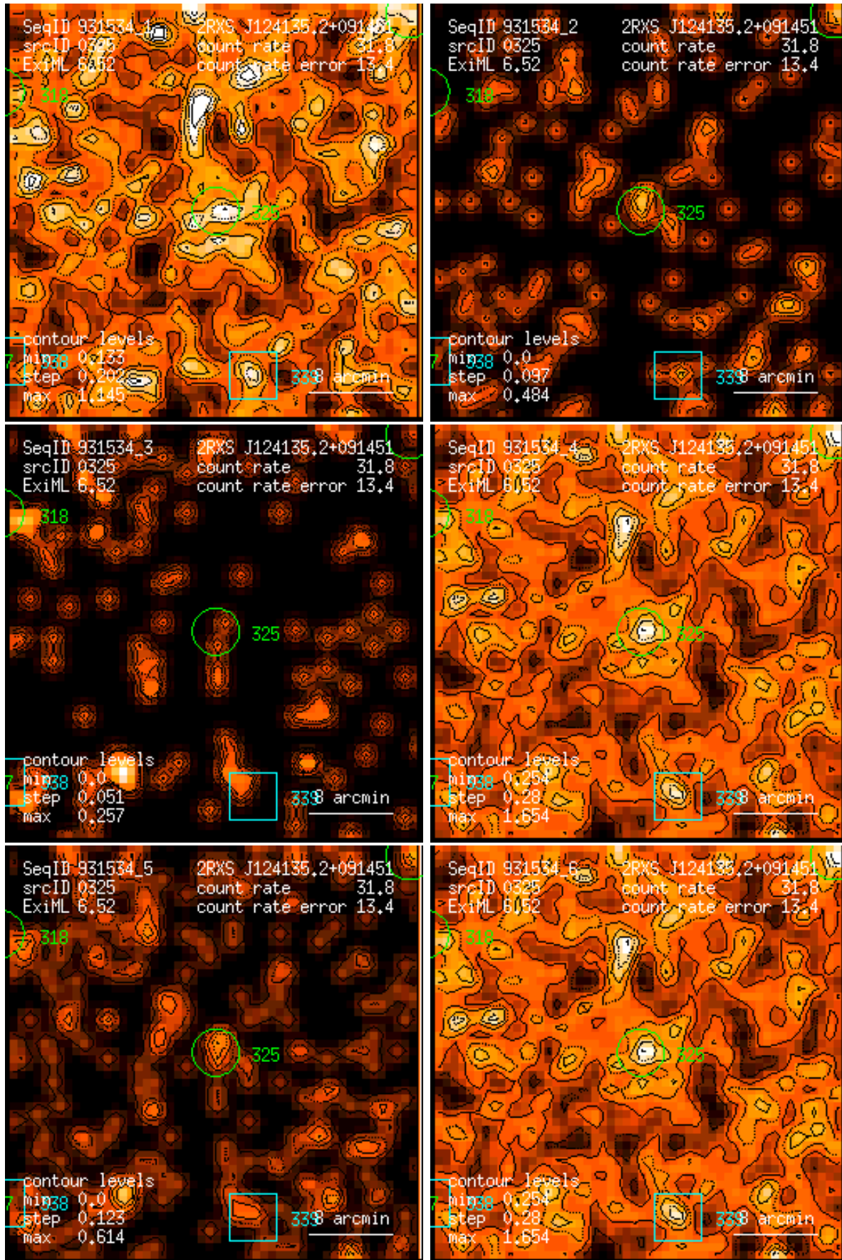
Figure 325: RASS 931534: detection 0325: band rate images, Gaussian filter: (1) PSPC channels 11 – 41, (2) 52 – 90, (3) 91 – 201, (4) 11 – 235, (5) 52 – 201, (6) 11 – 201. Broad band rates in counts/ks. Band rate contour levels in counts/ks/arcmin 2 .
