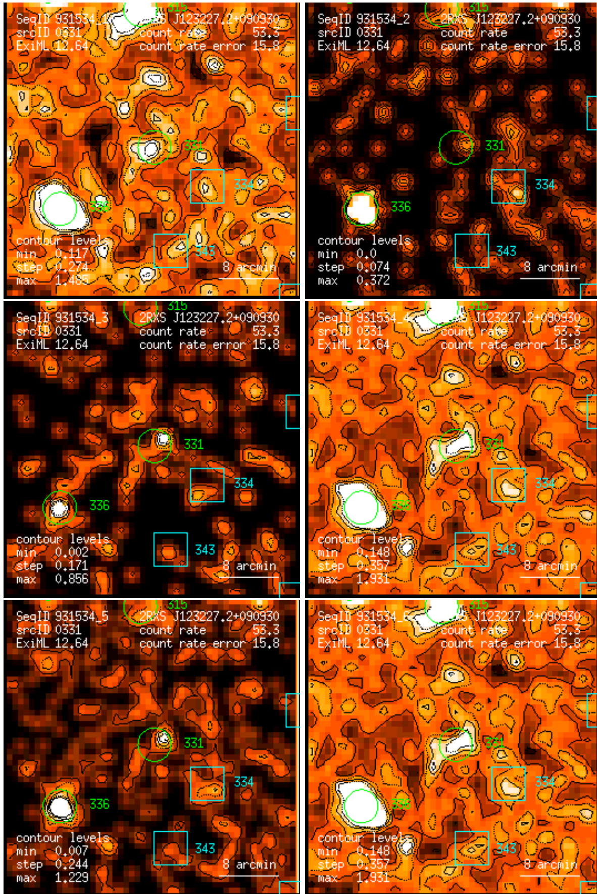
Figure 331: RASS 931534: detection 0331: band rate images, Gaussian filter: (1) PSPC channels 11 – 41, (2) 52 – 90, (3) 91 – 201, (4) 11 – 235, (5) 52 – 201, (6) 11 – 201. Broad band rates in counts/ks. Band rate contour levels in counts/ks/arcmin 2 .
