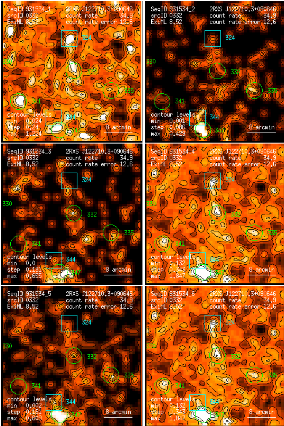
Figure 332: RASS 931534: detection 0332: band rate images, Gaussian filter: (1) PSPC channels 11 – 41, (2) 52 – 90, (3) 91 – 201, (4) 11 – 235, (5) 52 – 201, (6) 11 – 201. Broad band rates in counts/ks. Band rate contour levels in counts/ks/arcmin 2 .
