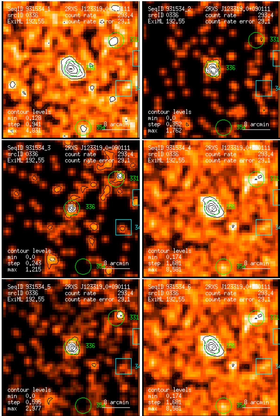
Figure 336: RASS 931534: detection 0336: band rate images, Gaussian filter: (1) PSPC channels 11 – 41, (2) 52 – 90, (3) 91 – 201, (4) 11 – 235, (5) 52 – 201, (6) 11 – 201. Broad band rates in counts/ks. Band rate contour levels in counts/ks/arcmin 2 .
