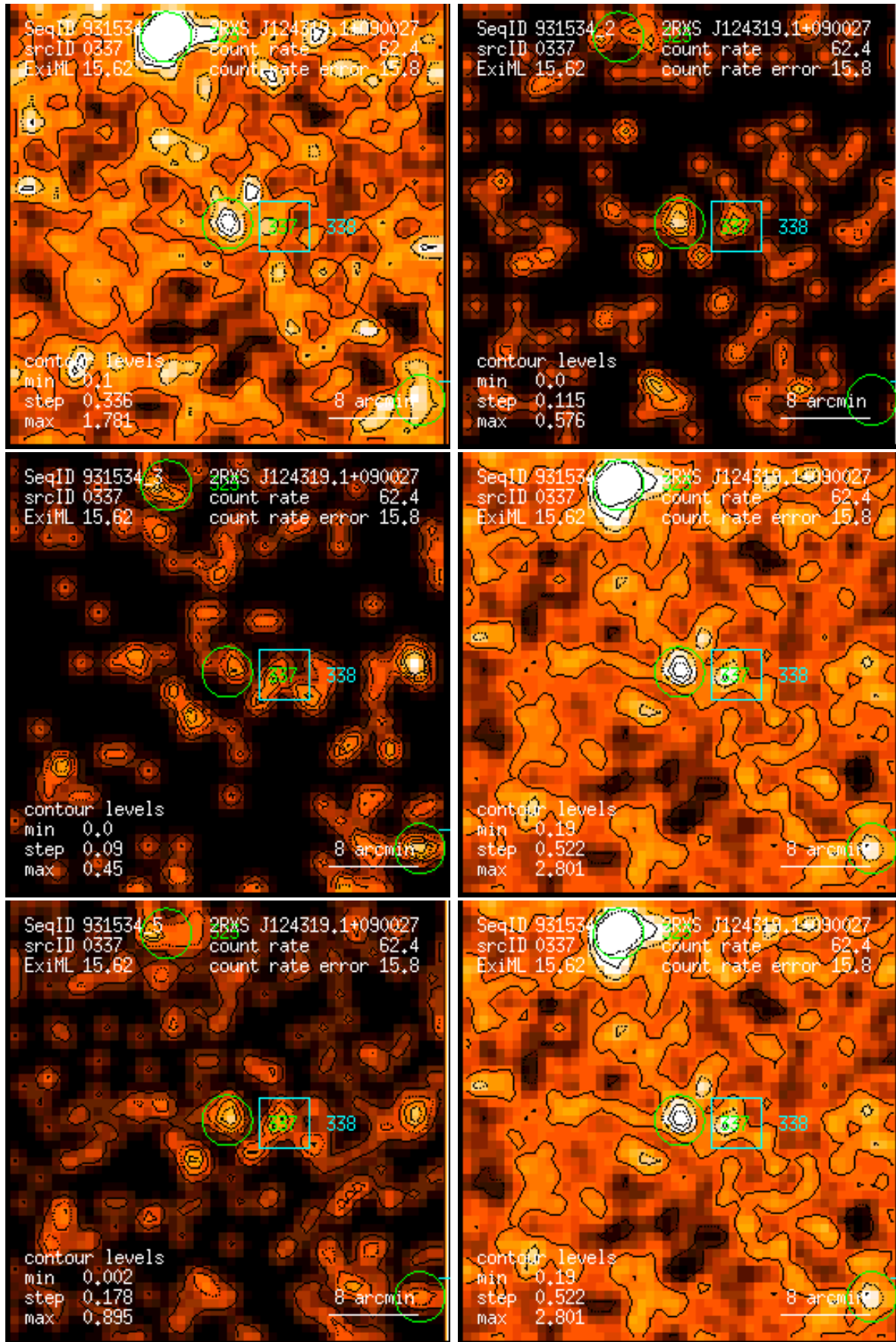
Figure 337: RASS 931534: detection 0337: band rate images, Gaussian filter: (1) PSPC channels 11 – 41, (2) 52 – 90, (3) 91 – 201, (4) 11 – 235, (5) 52 – 201, (6) 11 – 201. Broad band rates in counts/ks. Band rate contour levels in counts/ks/arcmin 2 .
