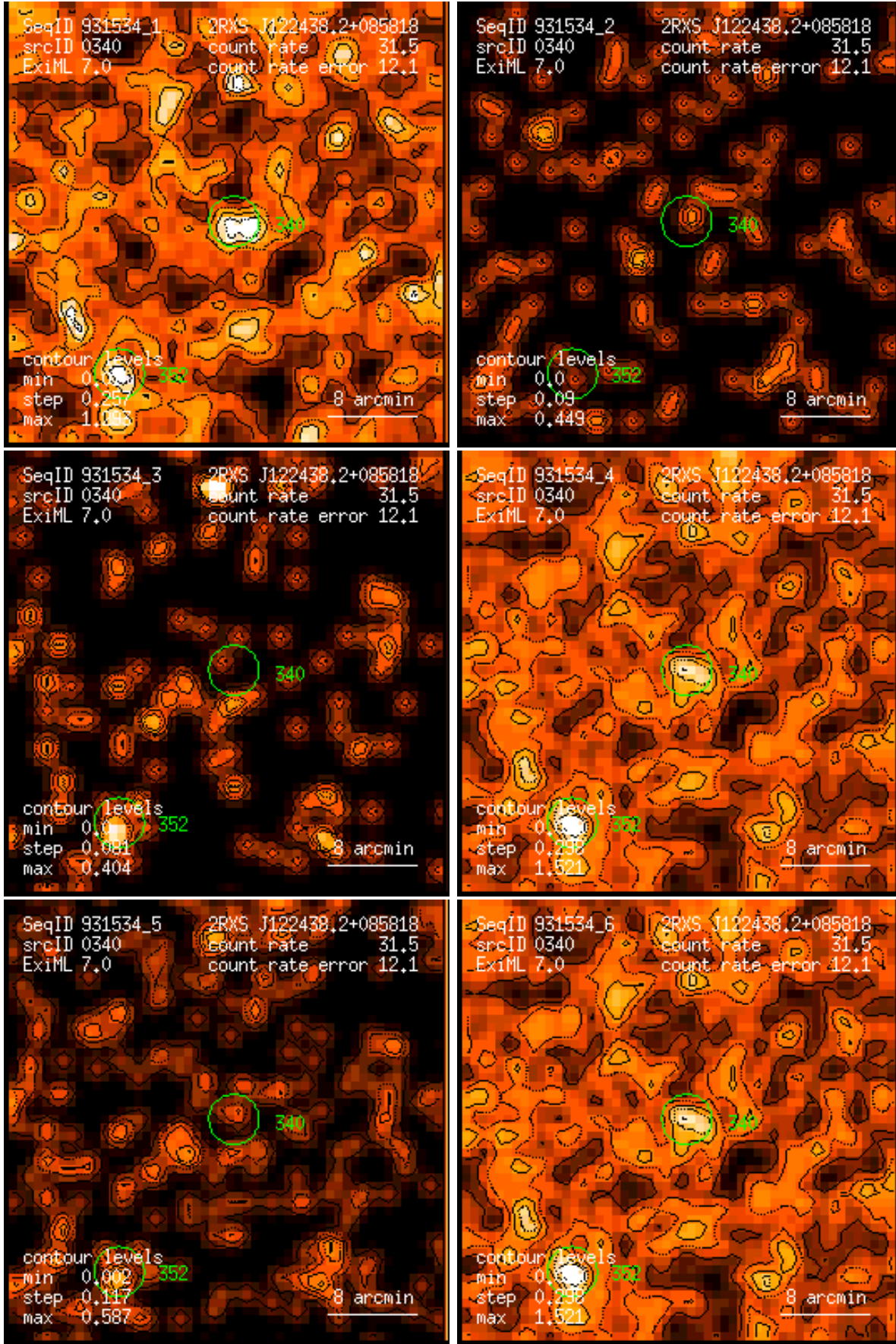
Figure 340: RASS 931534: detection 0340: band rate images, Gaussian filter: (1) PSPC channels 11 – 41, (2) 52 – 90, (3) 91 – 201, (4) 11 – 235, (5) 52 – 201, (6) 11 – 201. Broad band rates in counts/ks. Band rate contour levels in counts/ks/arcmin 2 .
