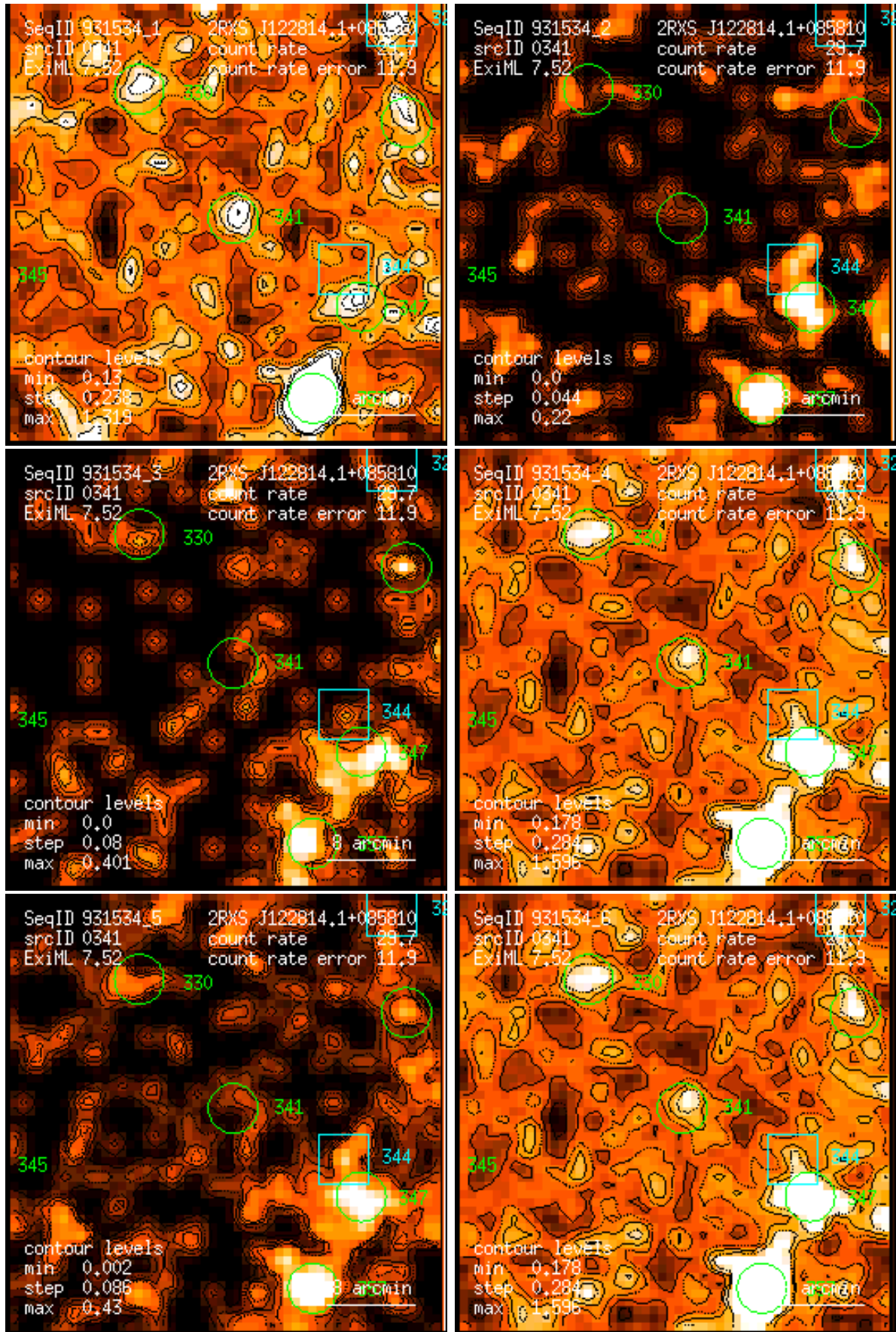
Figure 341: RASS 931534: detection 0341: band rate images, Gaussian filter: (1) PSPC channels 11 – 41, (2) 52 – 90, (3) 91 – 201, (4) 11 – 235, (5) 52 – 201, (6) 11 – 201. Broad band rates in counts/ks. Band rate contour levels in counts/ks/arcmin 2 .
