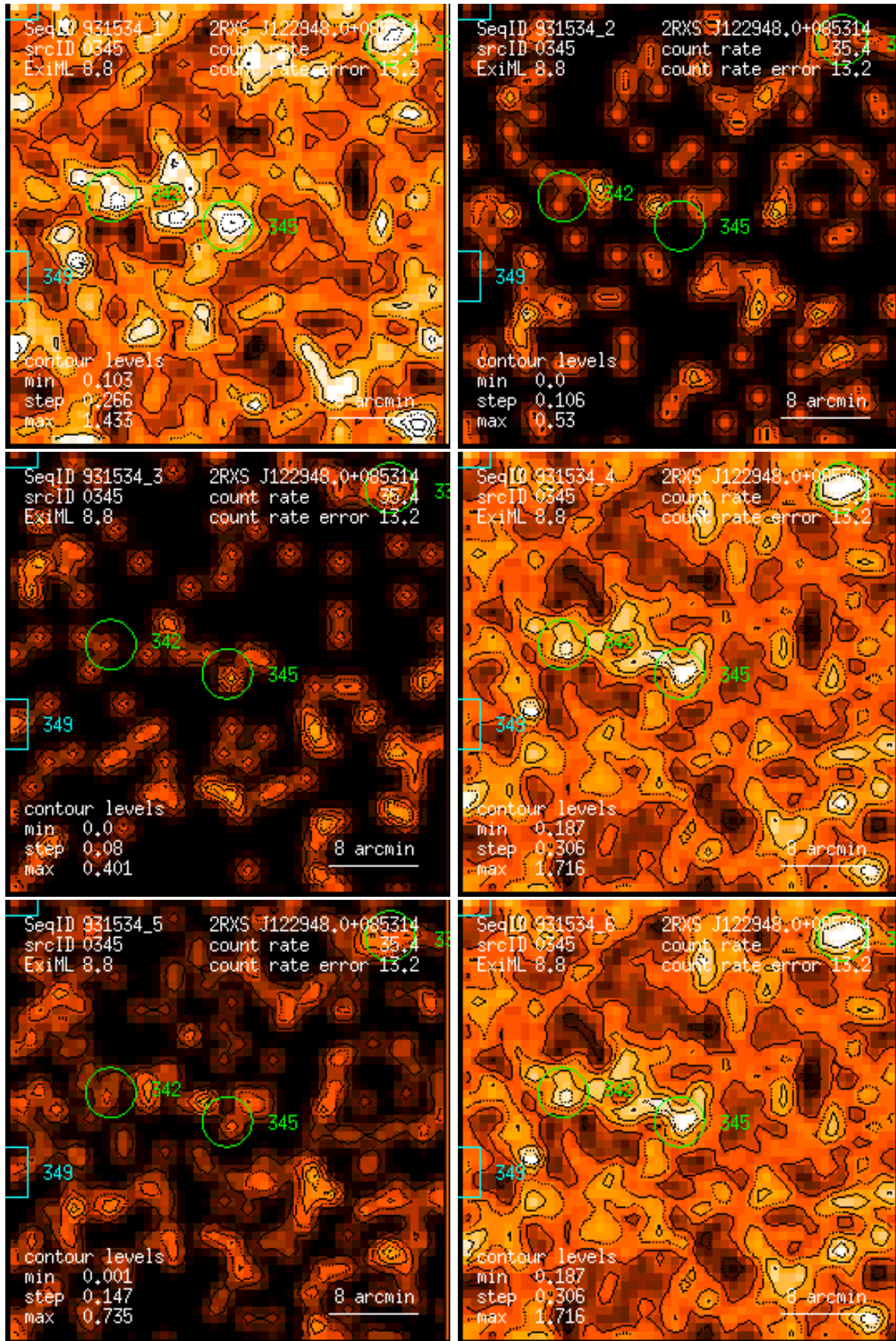
Figure 345: RASS 931534: detection 0345: band rate images, Gaussian filter: (1) PSPC channels 11 – 41, (2) 52 – 90, (3) 91 – 201, (4) 11 – 235, (5) 52 – 201, (6) 11 – 201. Broad band rates in counts/ks. Band rate contour levels in counts/ks/arcmin 2 .
