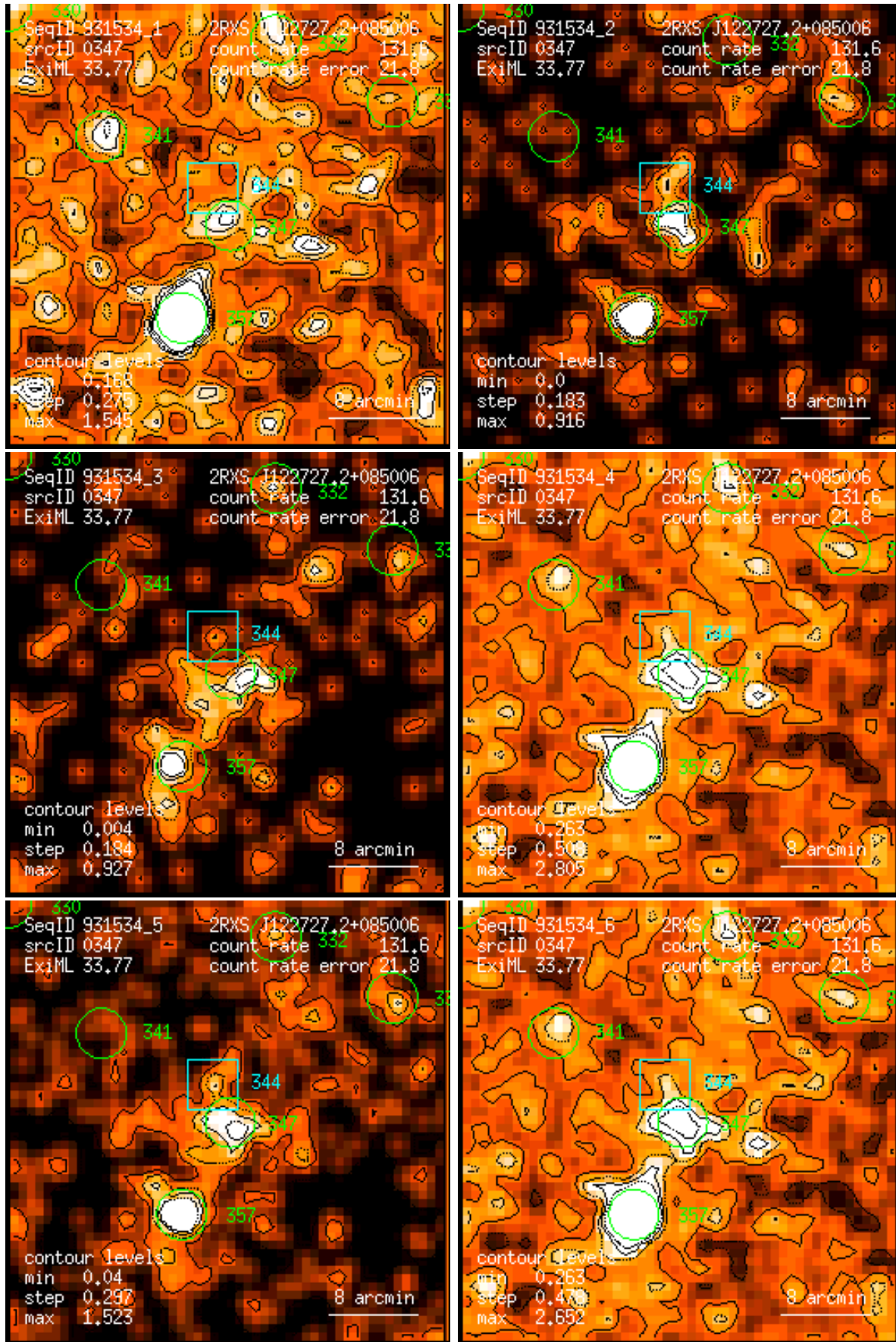
Figure 347: RASS 931534: detection 0347: band rate images, Gaussian filter: (1) PSPC channels 11 – 41, (2) 52 – 90, (3) 91 – 201, (4) 11 – 235, (5) 52 – 201, (6) 11 – 201. Broad band rates in counts/ks. Band rate contour levels in counts/ks/arcmin 2 .
