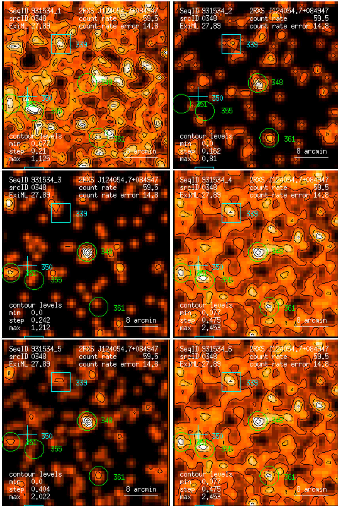
Figure 348: RASS 931534: detection 0348: band rate images, Gaussian filter: (1) PSPC channels 11 – 41, (2) 52 – 90, (3) 91 – 201, (4) 11 – 235, (5) 52 – 201, (6) 11 – 201. Broad band rates in counts/ks. Band rate contour levels in counts/ks/arcmin 2 .
