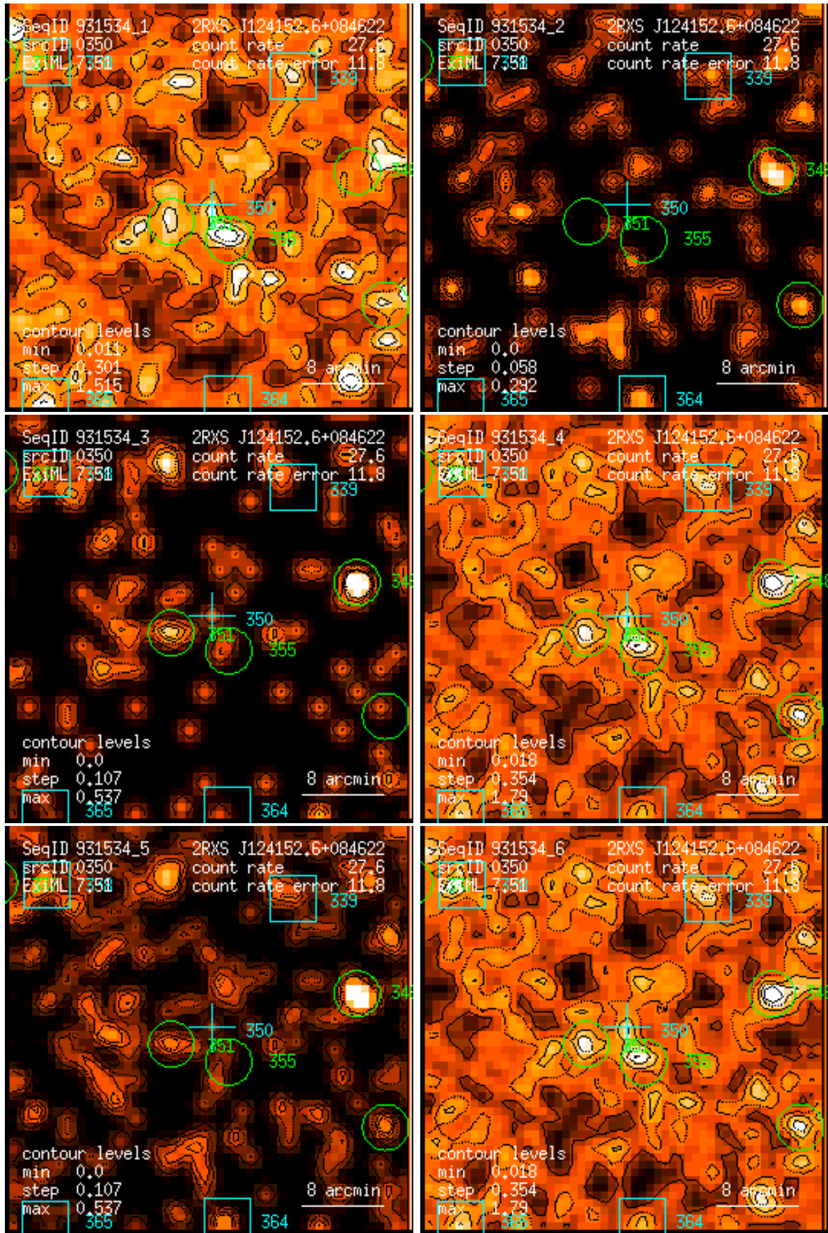
Figure 350: RASS 931534: detection 0350: band rate images, Gaussian filter: (1) PSPC channels 11 – 41, (2) 52 – 90, (3) 91 – 201, (4) 11 – 235, (5) 52 – 201, (6) 11 – 201. Broad band rates in counts/ks. Band rate contour levels in counts/ks/arcmin 2 .
