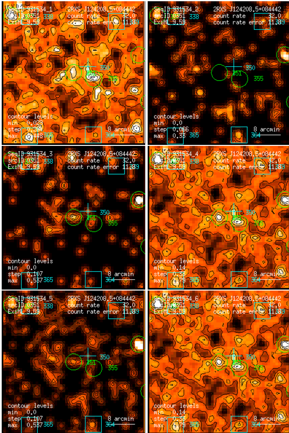
Figure 351: RASS 931534: detection 0351: band rate images, Gaussian filter: (1) PSPC channels 11 – 41, (2) 52 – 90, (3) 91 – 201, (4) 11 – 235, (5) 52 – 201, (6) 11 – 201. Broad band rates in counts/ks. Band rate contour levels in counts/ks/arcmin 2 .
