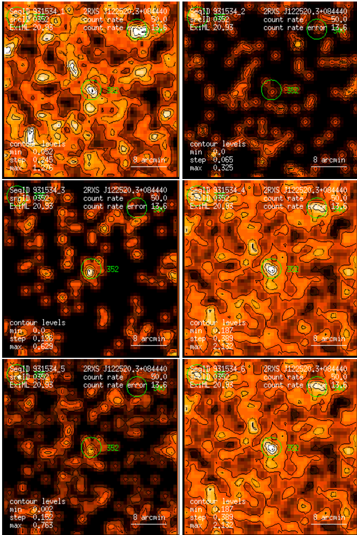
Figure 352: RASS 931534: detection 0352: band rate images, Gaussian filter: (1) PSPC channels 11 – 41, (2) 52 – 90, (3) 91 – 201, (4) 11 – 235, (5) 52 – 201, (6) 11 – 201. Broad band rates in counts/ks. Band rate contour levels in counts/ks/arcmin 2 .
