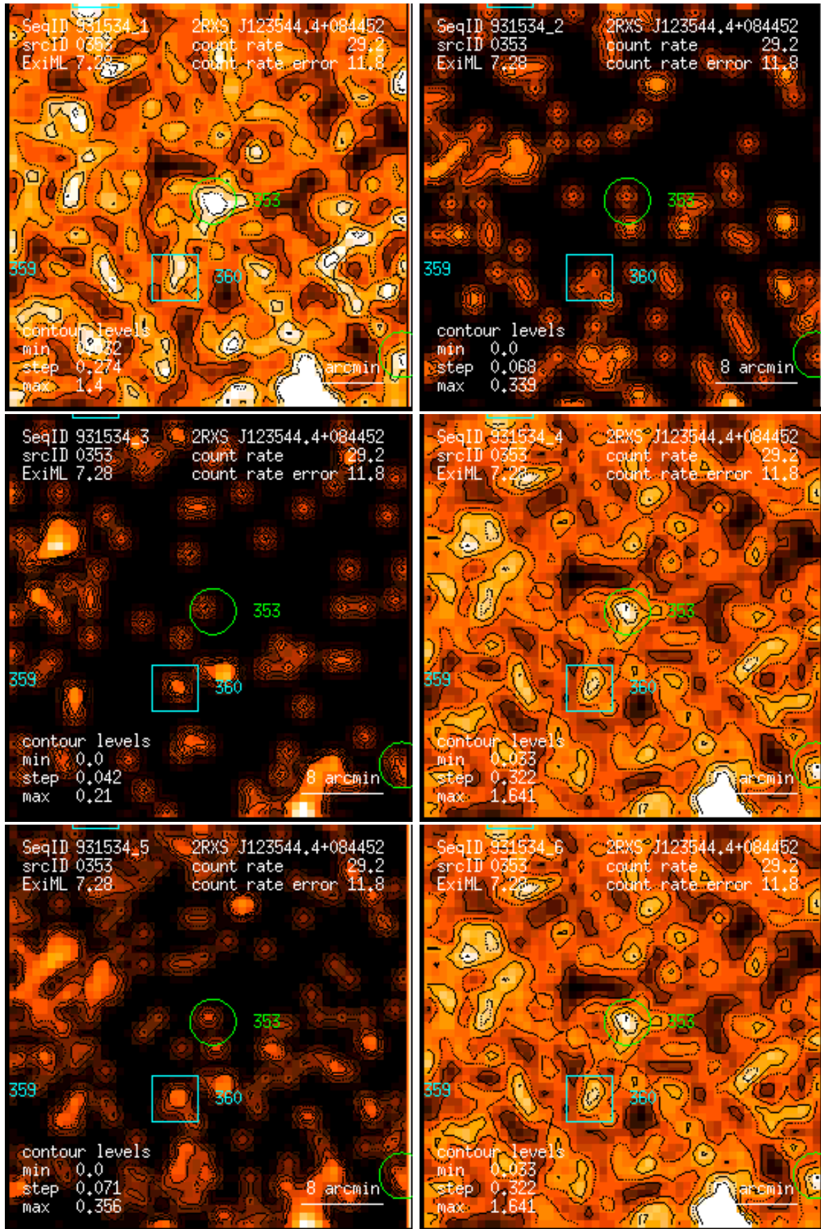
Figure 353: RASS 931534: detection 0353: band rate images, Gaussian filter: (1) PSPC channels 11 – 41, (2) 52 – 90, (3) 91 – 201, (4) 11 – 235, (5) 52 – 201, (6) 11 – 201. Broad band rates in counts/ks. Band rate contour levels in counts/ks/arcmin 2 .
