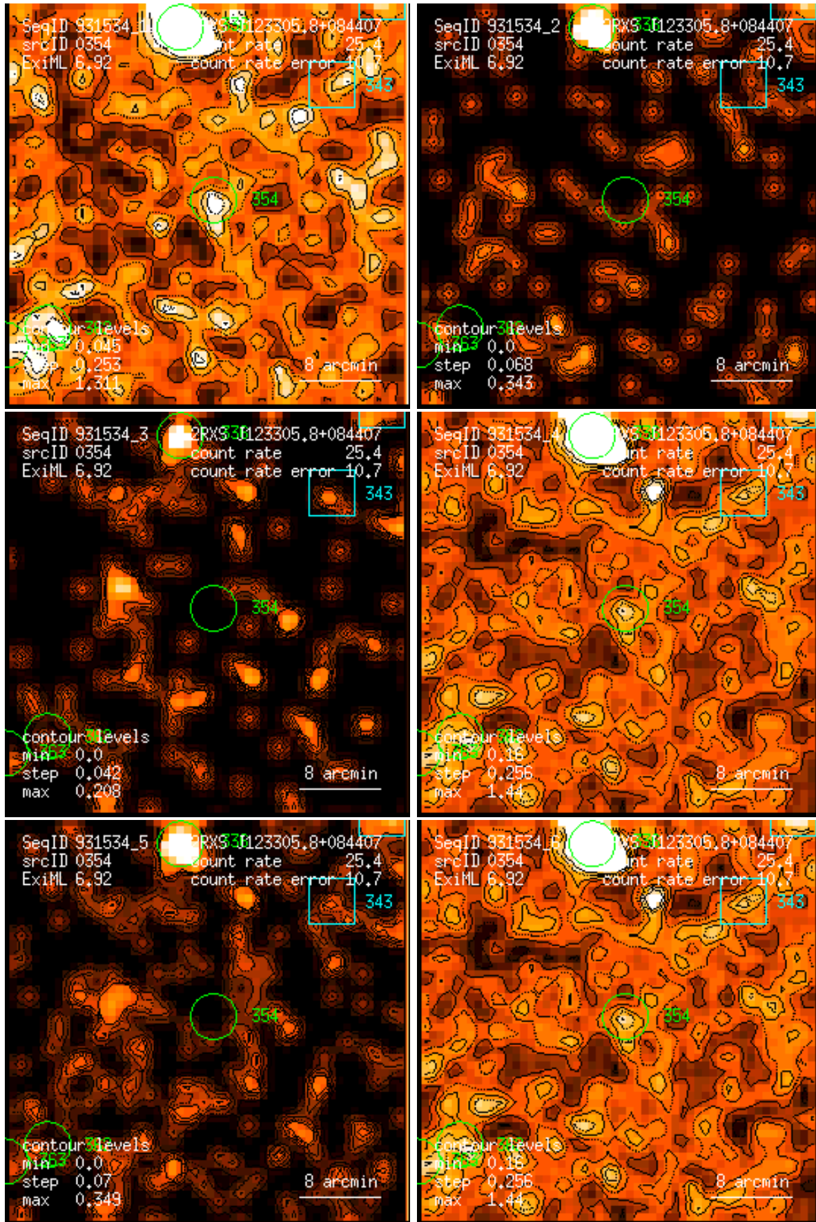
Figure 354: RASS 931534: detection 0354: band rate images, Gaussian filter: (1) PSPC channels 11 – 41, (2) 52 – 90, (3) 91 – 201, (4) 11 – 235, (5) 52 – 201, (6) 11 – 201. Broad band rates in counts/ks. Band rate contour levels in counts/ks/arcmin 2 .
