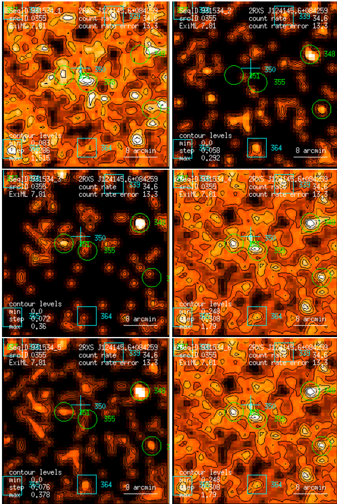
Figure 355: RASS 931534: detection 0355: band rate images, Gaussian filter: (1) PSPC channels 11 – 41, (2) 52 – 90, (3) 91 – 201, (4) 11 – 235, (5) 52 – 201, (6) 11 – 201. Broad band rates in counts/ks. Band rate contour levels in counts/ks/arcmin 2 .
