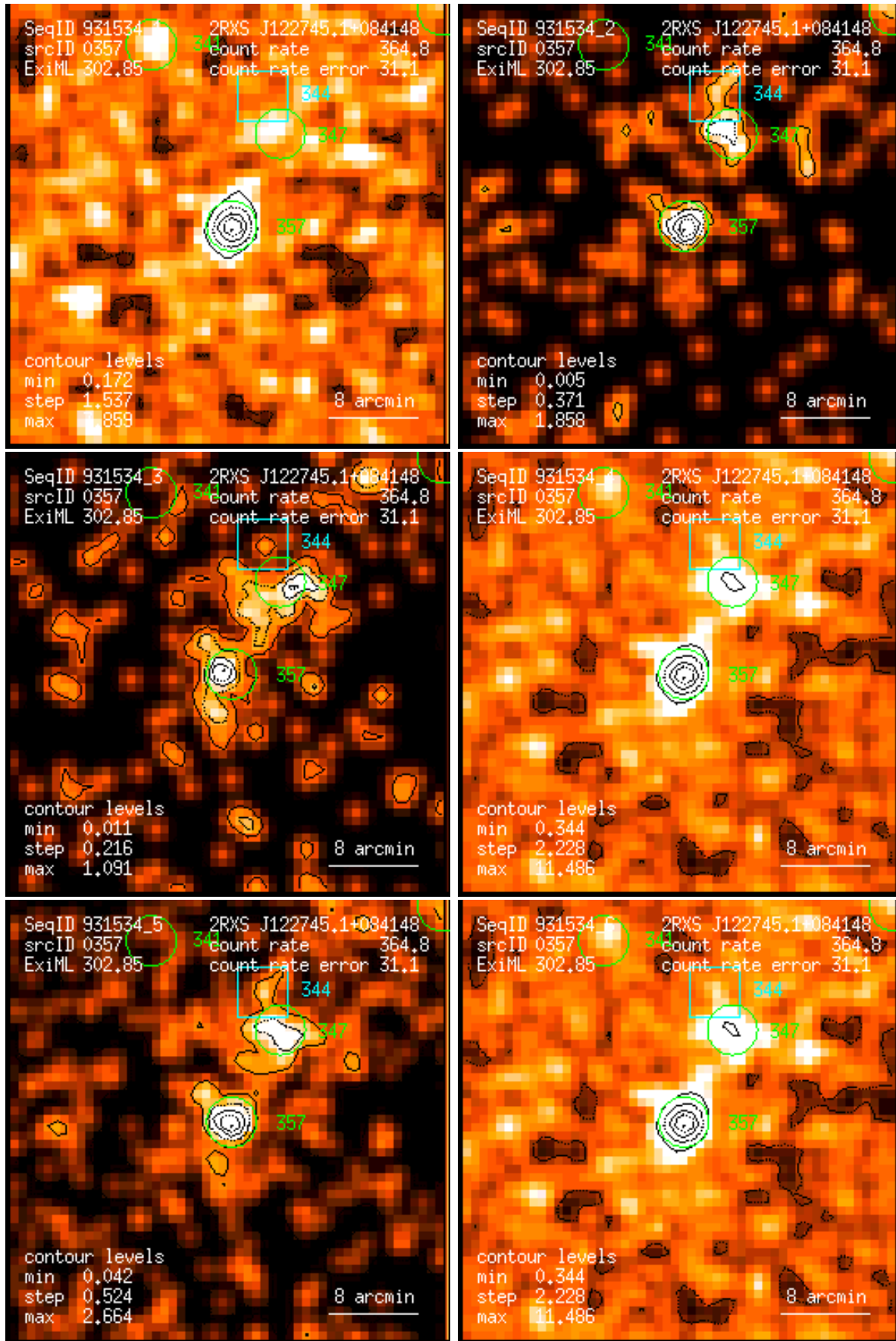
Figure 357: RASS 931534: detection 0357: band rate images, Gaussian filter: (1) PSPC channels 11 – 41, (2) 52 – 90, (3) 91 – 201, (4) 11 – 235, (5) 52 – 201, (6) 11 – 201. Broad band rates in counts/ks. Band rate contour levels in counts/ks/arcmin 2 .
