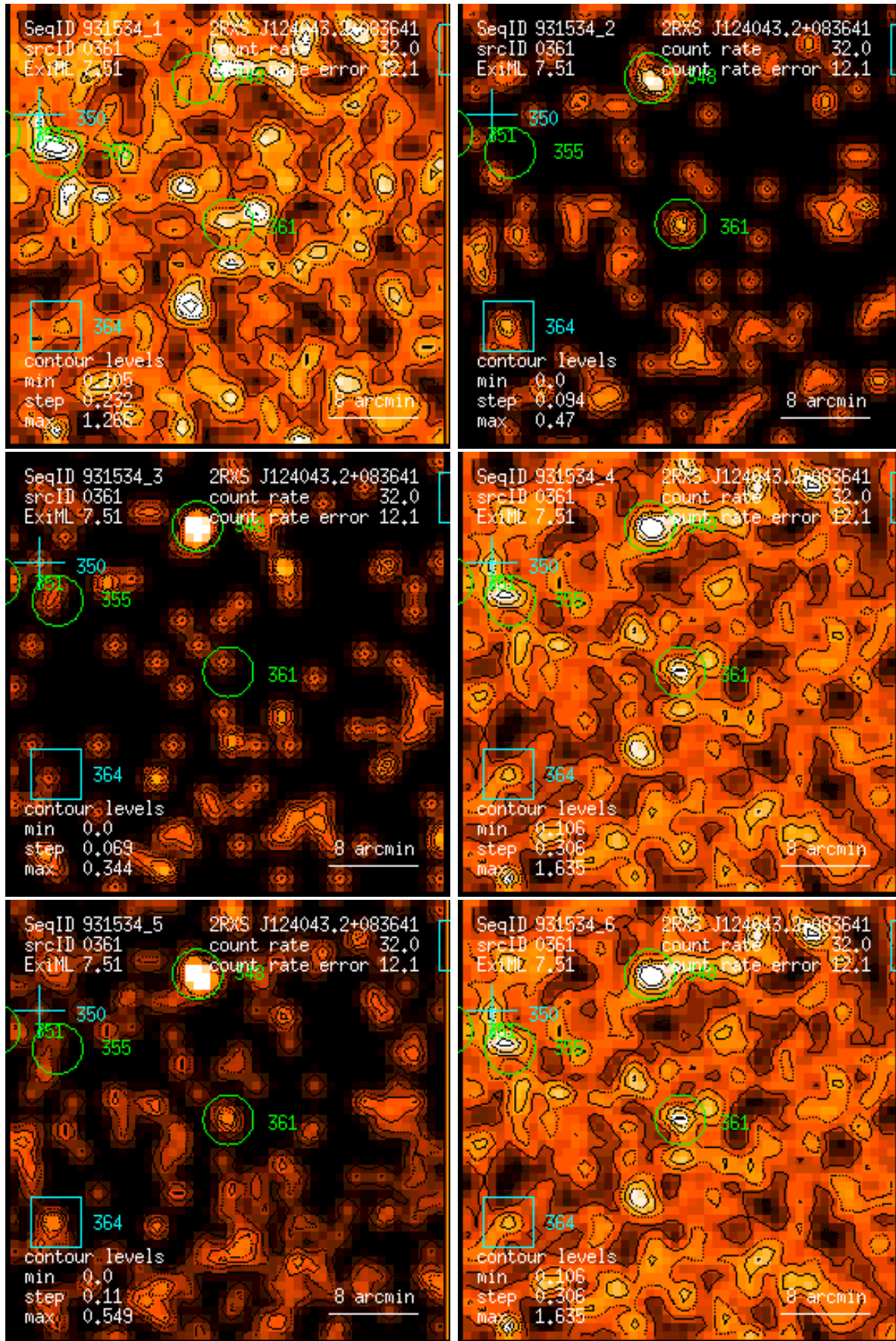
Figure 361: RASS 931534: detection 0361: band rate images, Gaussian filter: (1) PSPC channels 11 – 41, (2) 52 – 90, (3) 91 – 201, (4) 11 – 235, (5) 52 – 201, (6) 11 – 201. Broad band rates in counts/ks. Band rate contour levels in counts/ks/arcmin 2 .
