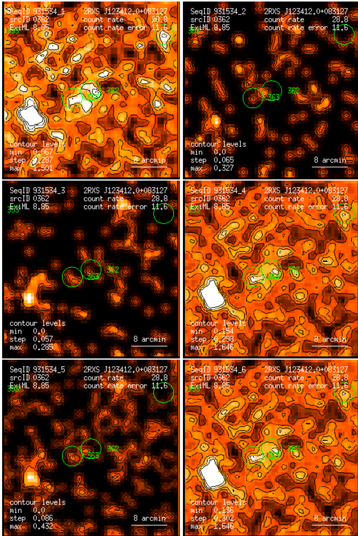
Figure 362: RASS 931534: detection 0362: band rate images, Gaussian filter: (1) PSPC channels 11 – 41, (2) 52 – 90, (3) 91 – 201, (4) 11 – 235, (5) 52 – 201, (6) 11 – 201. Broad band rates in counts/ks. Band rate contour levels in counts/ks/arcmin 2 .
